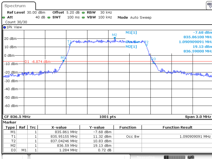
Band5-1.4MHz-QPSK-20525-6RB#0-1.091
