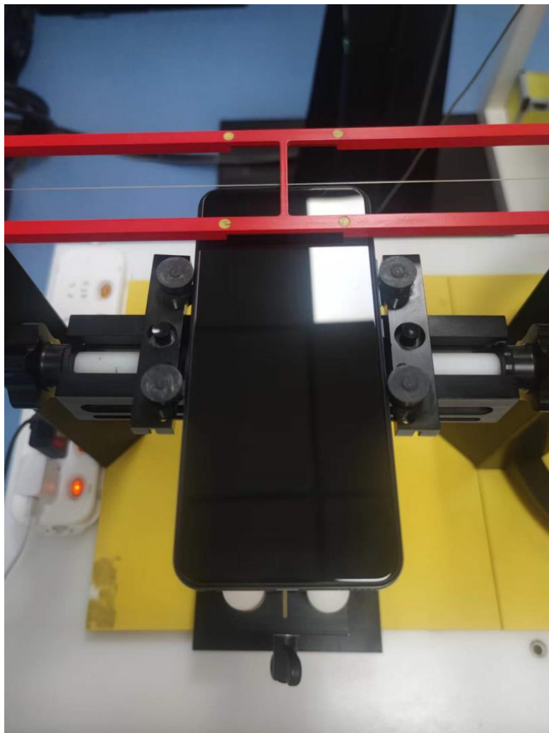
Picture 2: EUT Positioning for RF/T-coil
