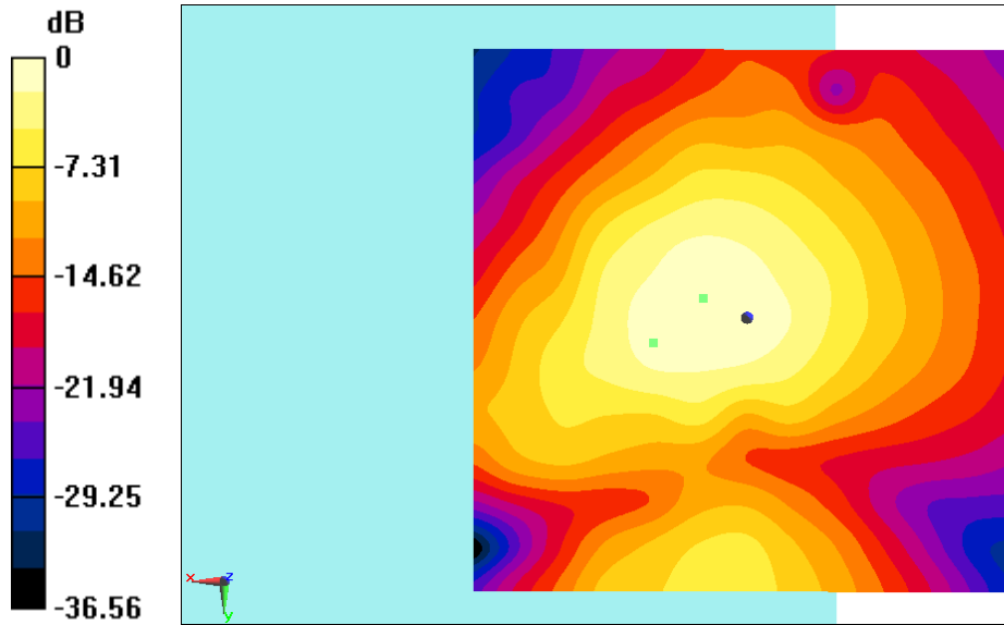
Fig B.1 T-Coil WiFi5G
