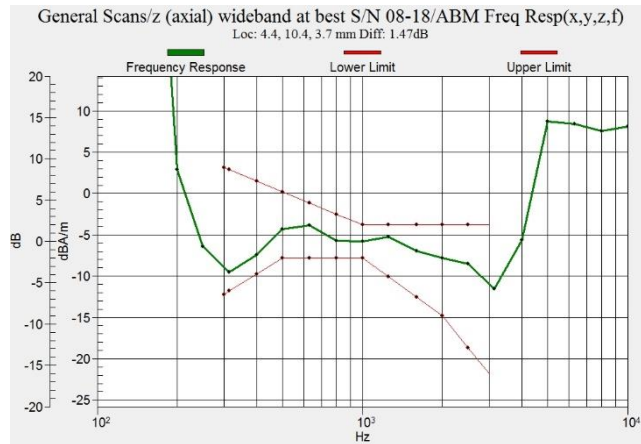
Figure C.1 Frequency Response of LTEB30
