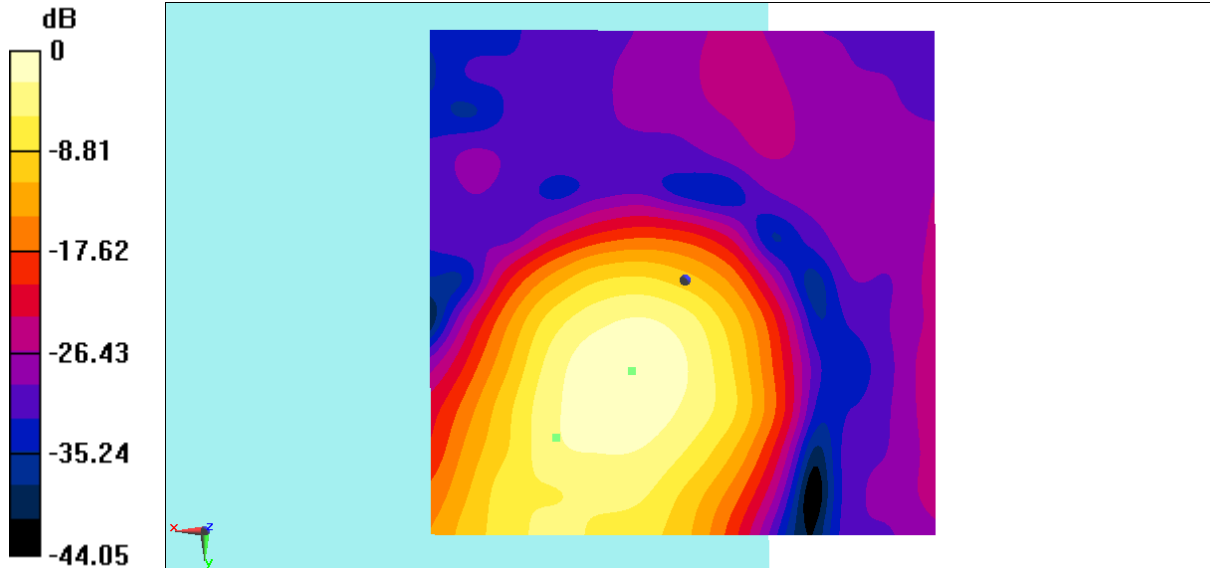
Fig B.4 T-Coil LTEB30
