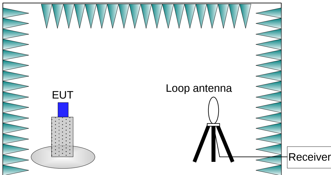
Figure B-3: Measurement Setup
