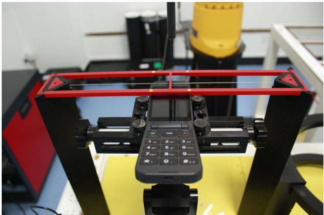
Picture 2: EUT Positioning for T-coil
