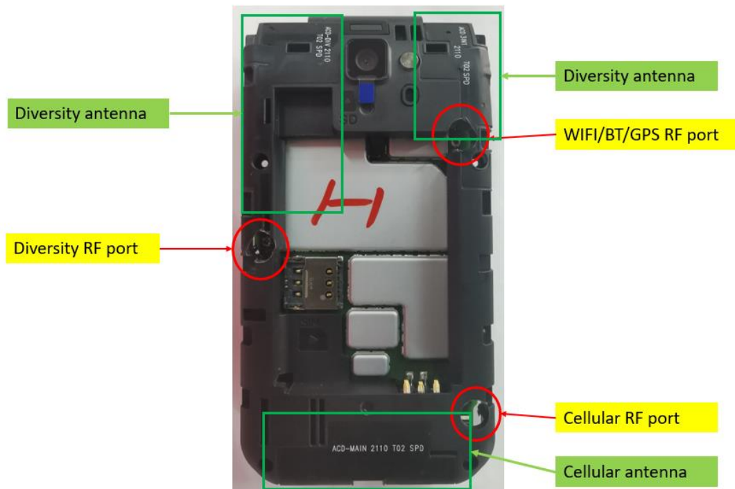
Picture 9: Antenna locations
