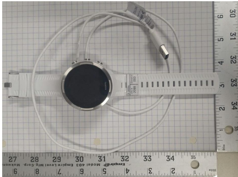
Figure B1. Front of DUT with Charging Cable connected
