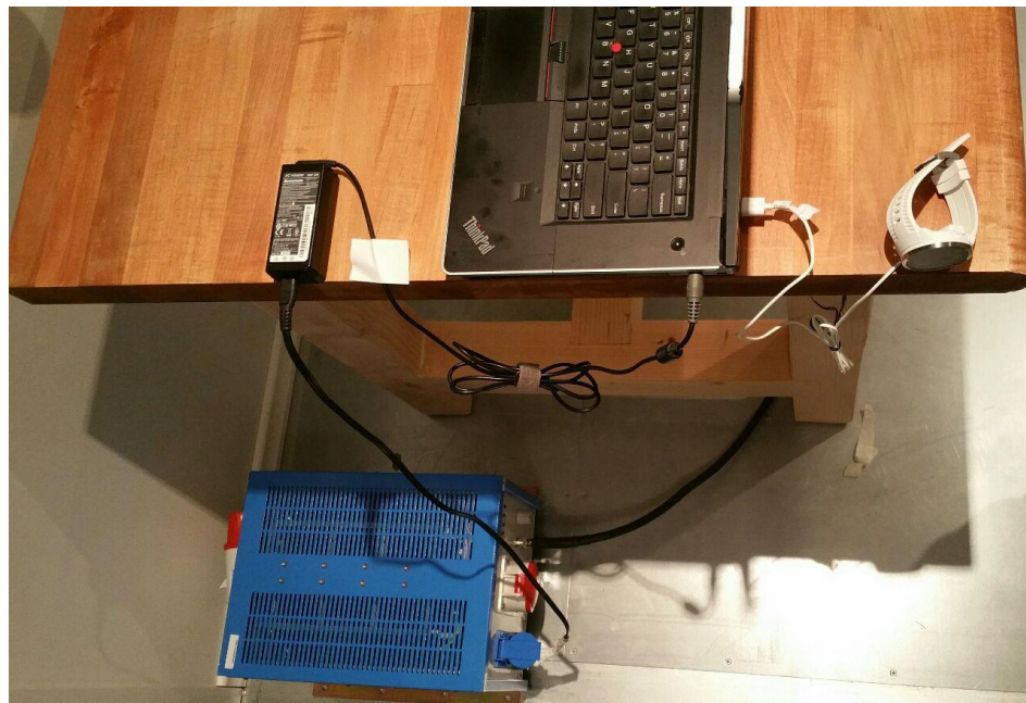
Figure B5: Conducted Emission Set up
