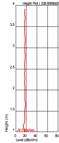
Height Plot ( 238.69592056 MHz )
