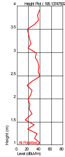
Height Plot ( 195.137475028 MHz )
