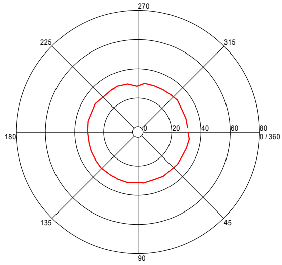
Turntable Plot ( 30.421242597 MHz )
