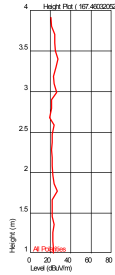
Height Plot ( 167.460320521 MHz )
