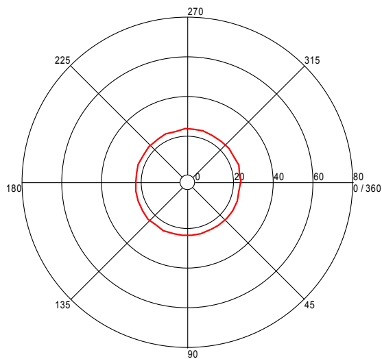
Turntable Plot ( 167.166132144 MHz )
