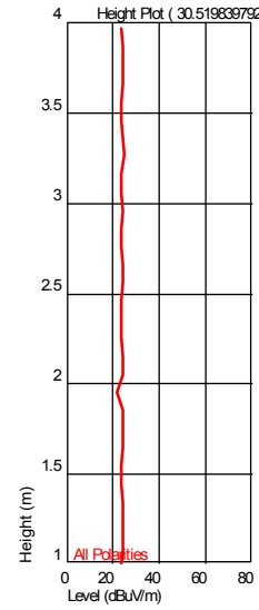
Height Plot ( 30.519839792 MHz )
