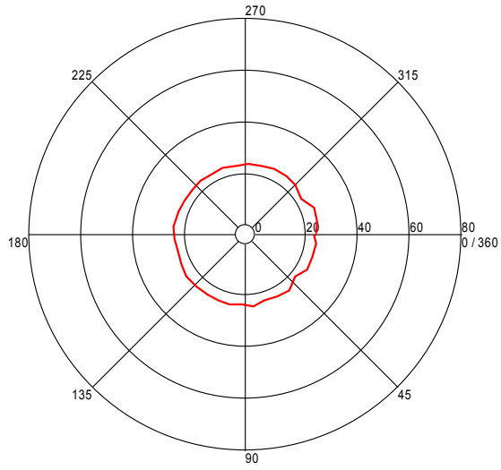
Turntable Plot ( 30.519839792 MHz )
