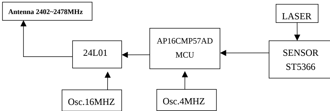
Block Diagram
