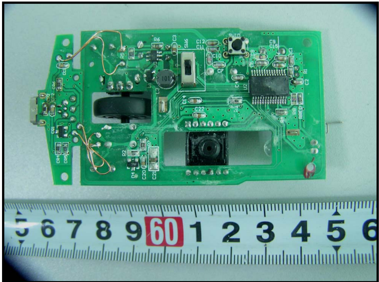
EUT- Main Board Components Bottom View
