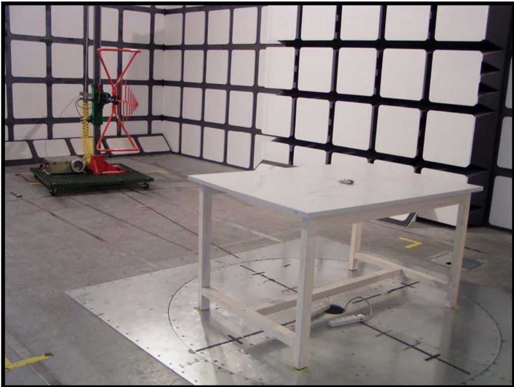
Radiated Emissions - Rear View (above 30 MHz)
