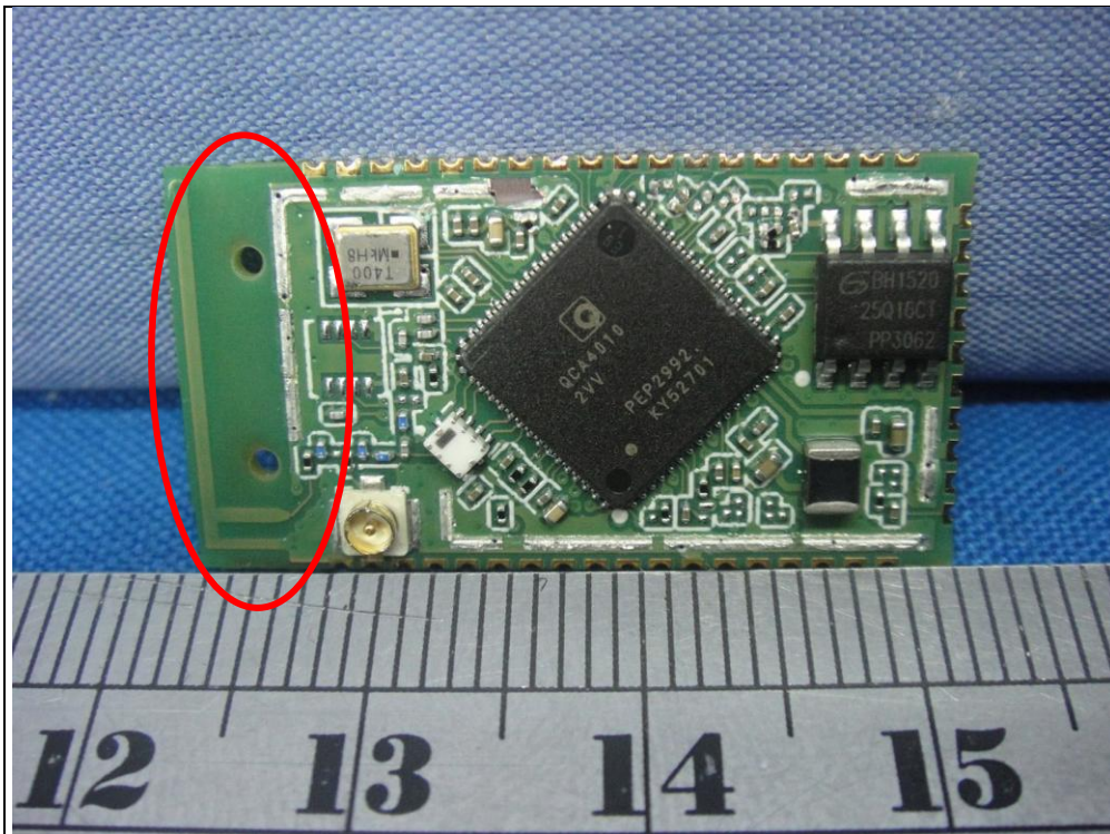
Antenna (Brand: QCA, Model: MP1-2.4GANT)
