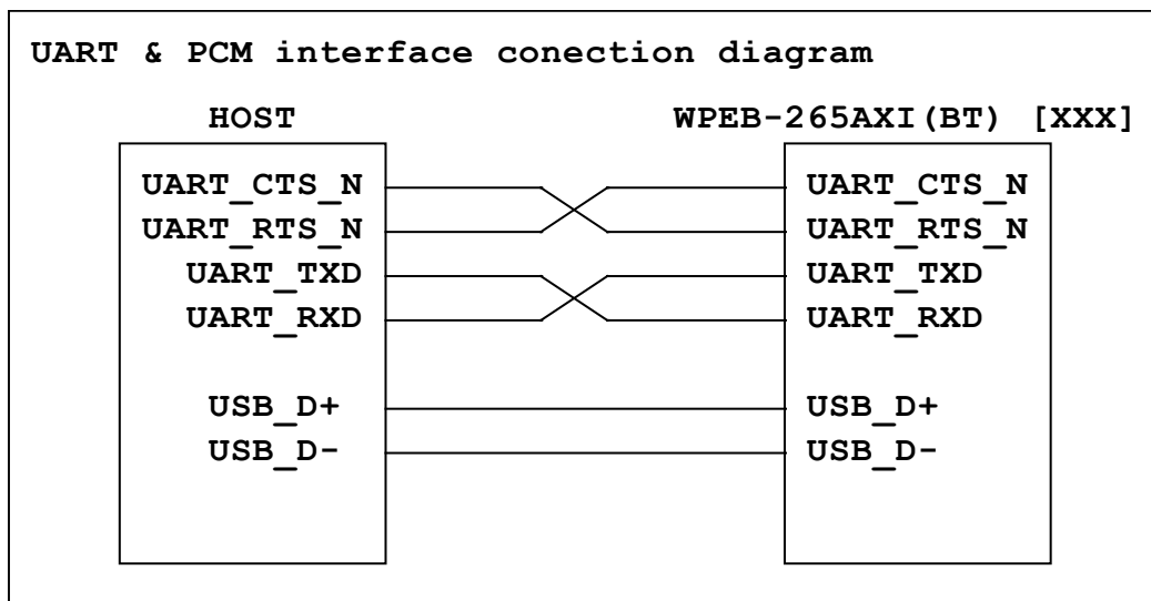
Figure4. UART and USB Interface Connection Diagram
