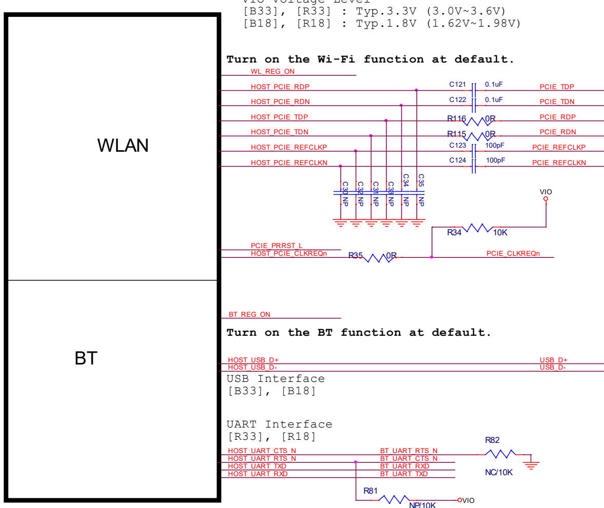
Figure2. External Reference Circuit
