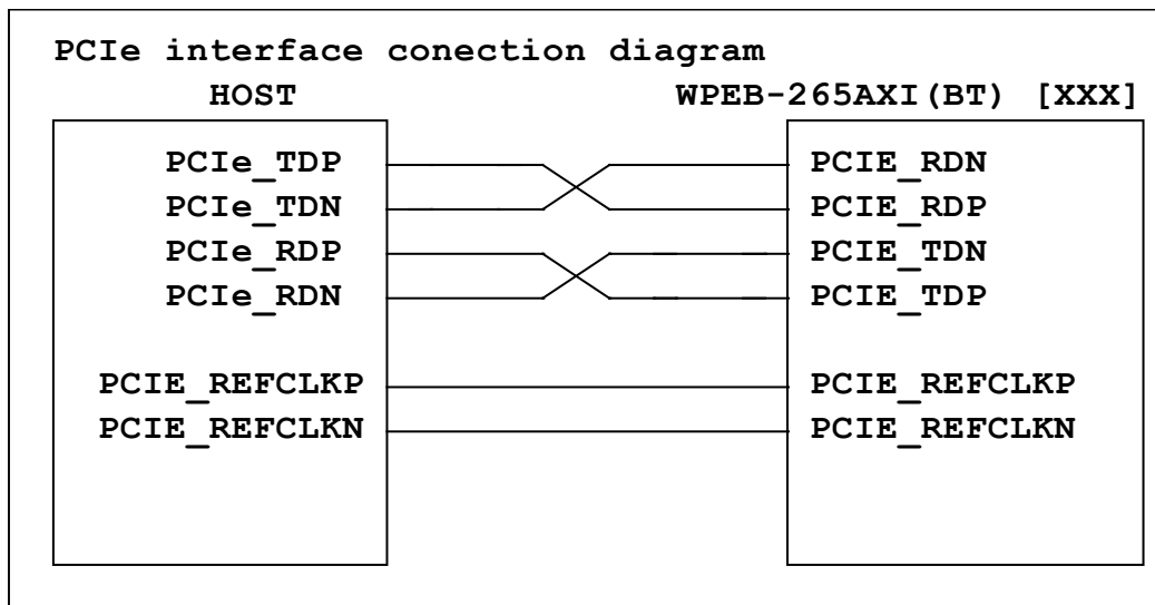
Figure3. PCI-e Interface Connection Diagram
