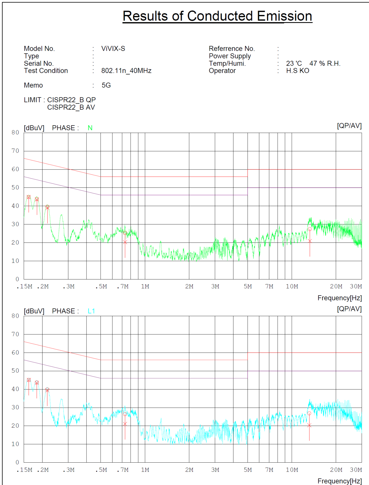
Figure.3. Conducted Emissions Graph
