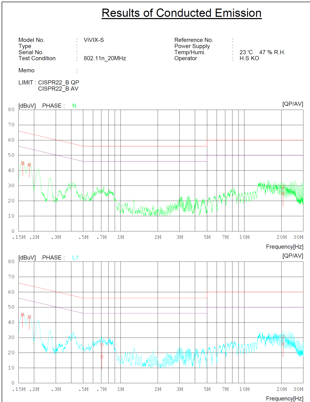
Figure.2. Conducted Emissions Graph
