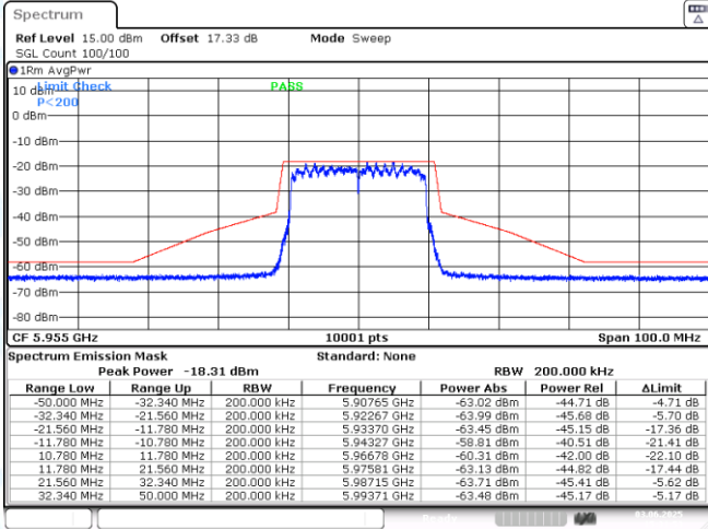
NTNV-11AX20MIMO-Ant1-5955-PASS
