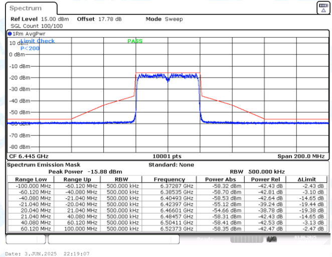
NTNV-11AX40MIMO-Ant2-6445-PASS
