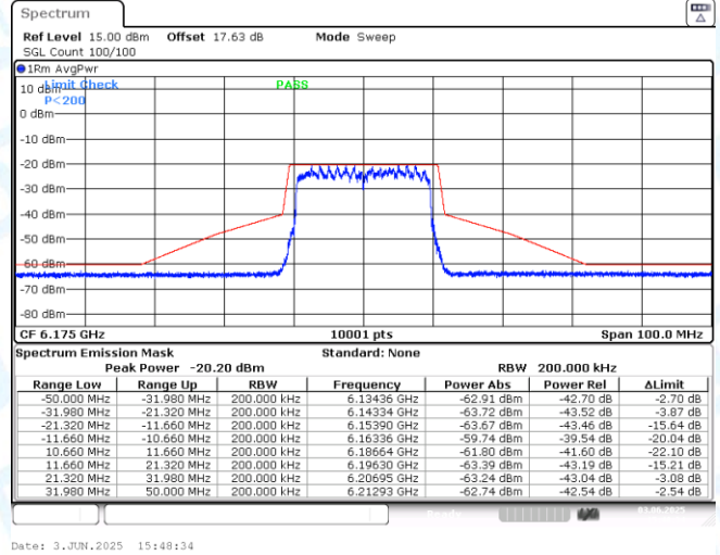
NTNV-11AX20MIMO-Ant2-6175-PASS
