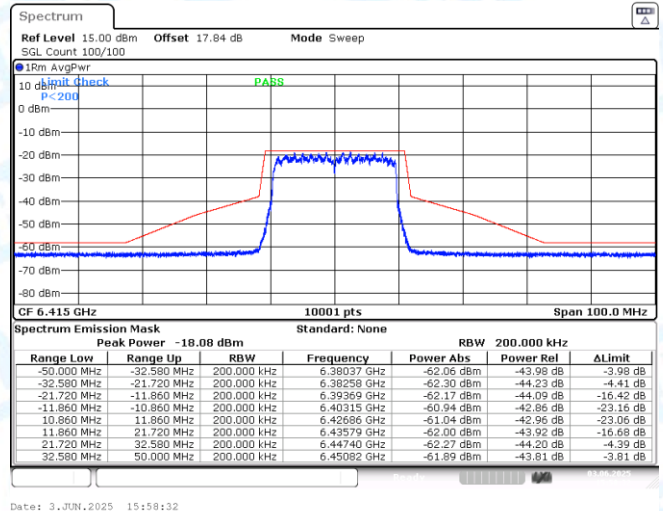
NTNV-11AX20MIMO-Ant2-6415-PASS
