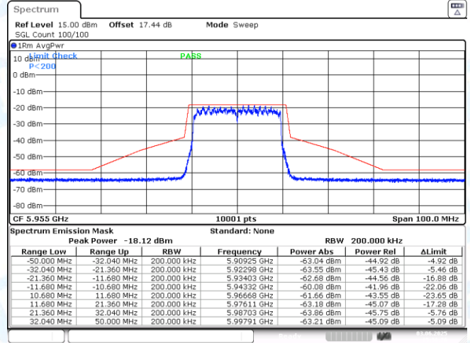
NTNV-11AX20MIMO-Ant2-5955-PASS
