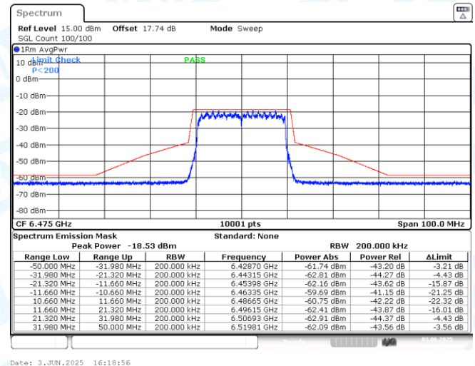
NTNV-11AX20MIMO-Ant2-6475-PASS
