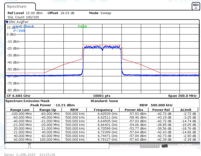
NTNV-11AX40MIMO-Ant2-6685-PASS
