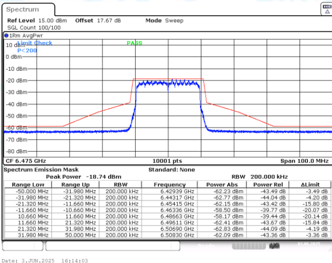
NTNV-11AX20MIMO-Ant1-6475-PASS
