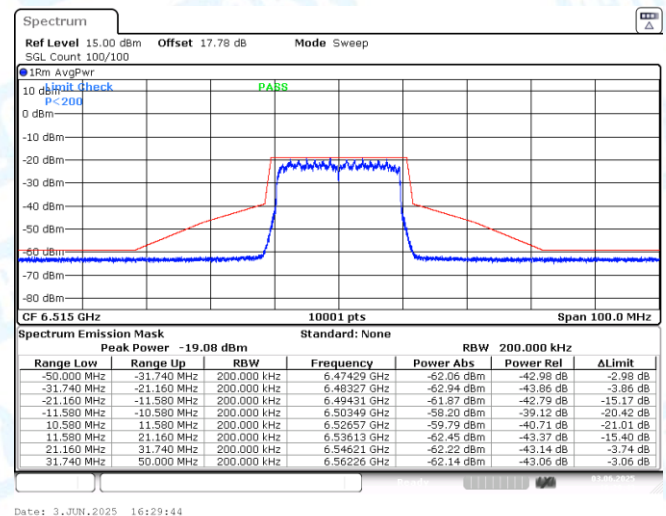
NTNV-11AX20MIMO-Ant2-6515-PASS
