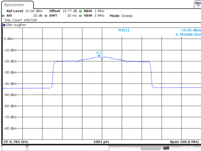
11AX80MIMO-Ant1-6785-PASS
