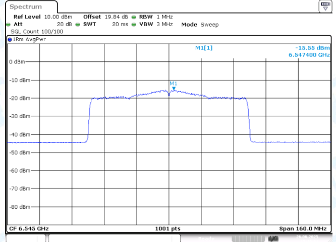
11AX80MIMO-Ant2-6545-PASS
