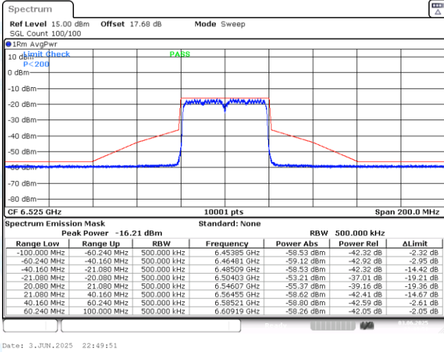
NTNV-11AX40MIMO-Ant1-6525-PASS
