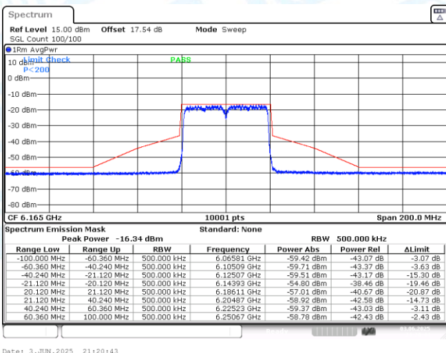
NTNV-11AX40MIMO-Ant1-6165-PASS
