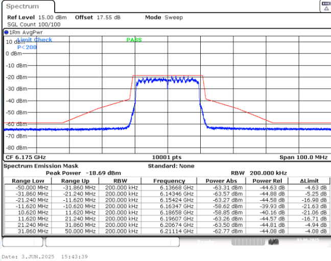
NTNV-11AX20MIMO-Ant1-6175-PASS
