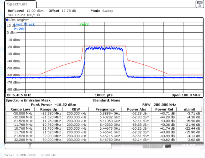
NTNV-11AX20MIMO-Ant2-6435-PASS
