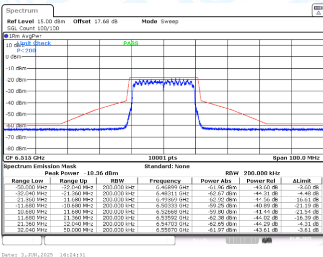
NTNV-11AX20MIMO-Ant1-6515-PASS
