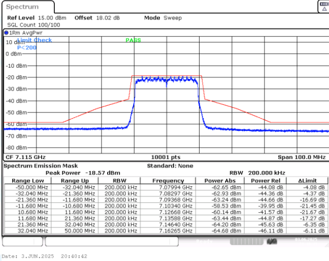
NTNV-11AX20MIMO-Ant1-7115-PASS
