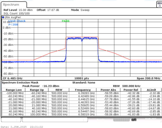
NTNV-11AX40MIMO-Ant1-6485-PASS
