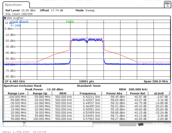
NTNV-11AX40MIMO-Ant2-6485-PASS
