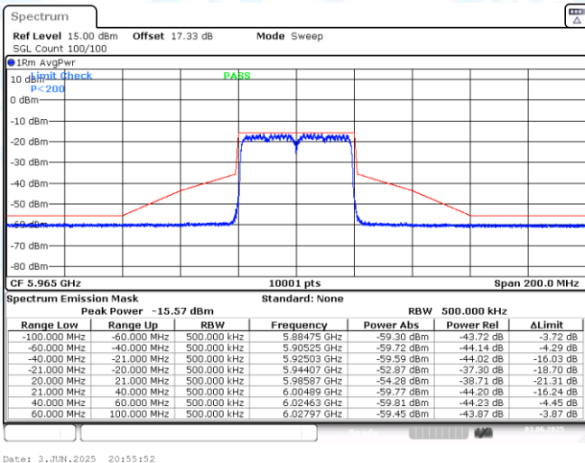
NTNV-11AX40MIMO-Ant1-5965-PASS
