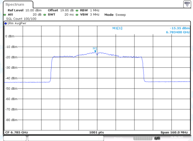
11AX80MIMO-Ant2-6785-PASS
