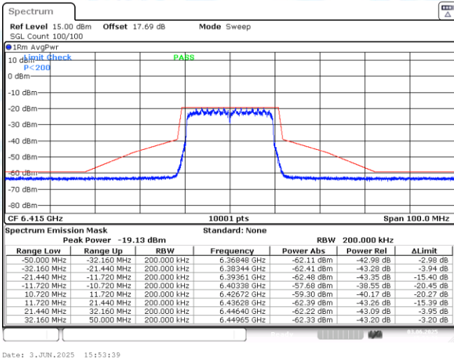
NTNV-11AX20MIMO-Ant1-6415-PASS
