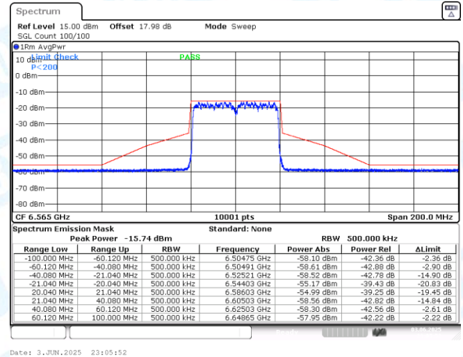
NTNV-11AX40MIMO-Ant2-6565-PASS
