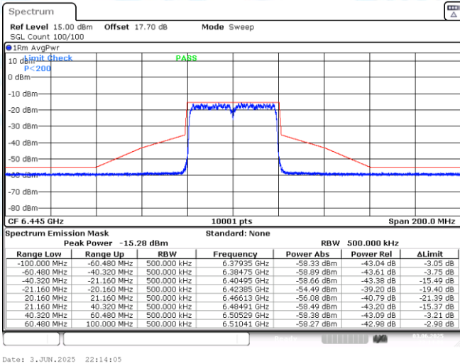
NTNV-11AX40MIMO-Ant1-6445-PASS
