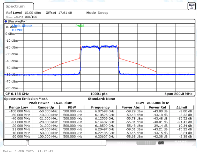
NTNV-11AX40MIMO-Ant2-6165-PASS
