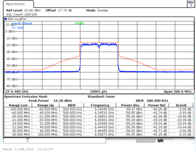
NTNV-11AX40MIMO-Ant2-6405-PASS
