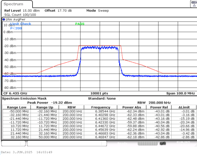
NTNV-11AX20MIMO-Ant1-6435-PASS
