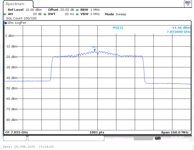
11AX80MIMO-Ant2-7025-PASS
