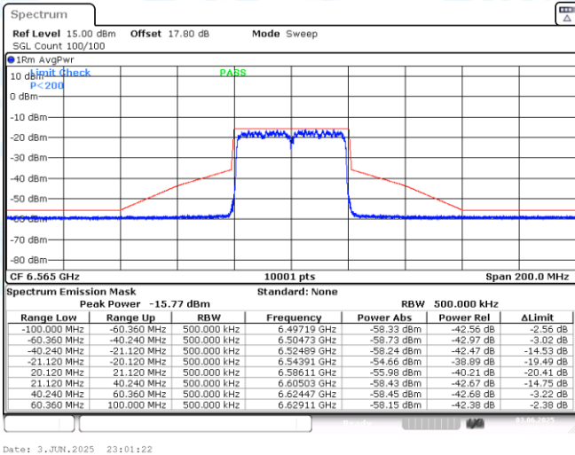
NTNV-11AX40MIMO-Ant1-6565-PASS
