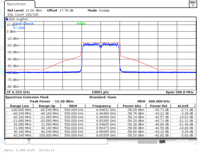
NTNV-11AX40MIMO-Ant2-6525-PASS
