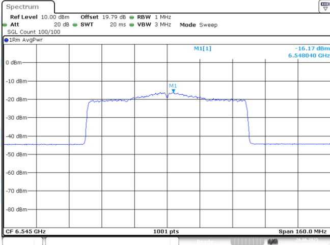
11AX80MIMO-Ant1-6545-PASS
