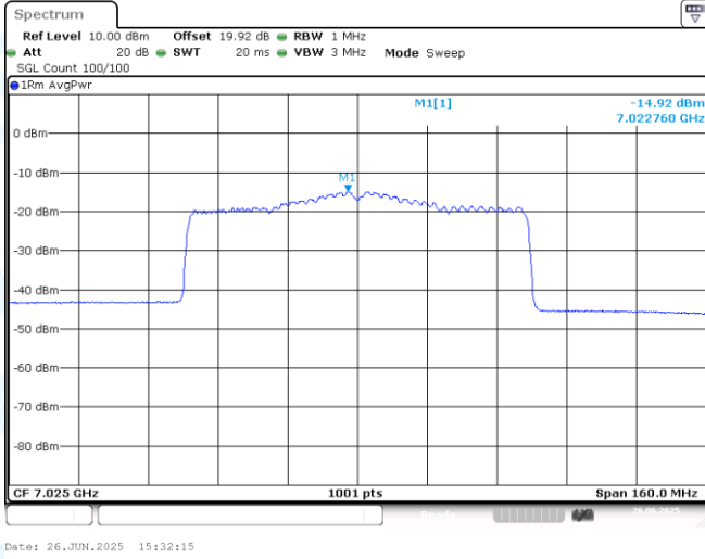
11AX80MIMO-Ant1-7025-PASS
