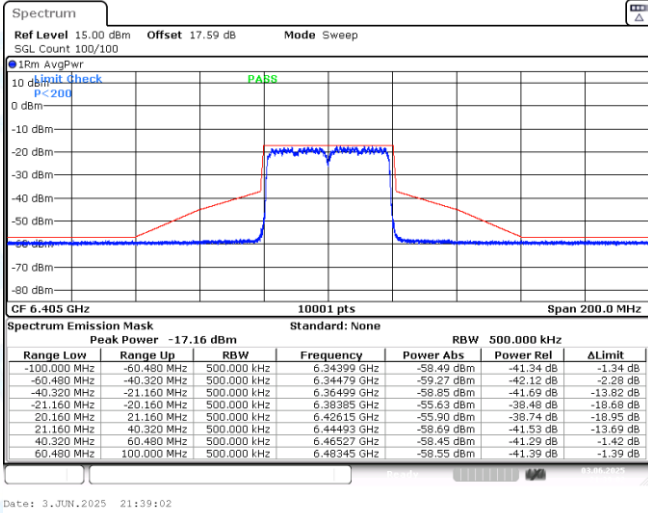
NTNV-11AX40MIMO-Ant1-6405-PASS
