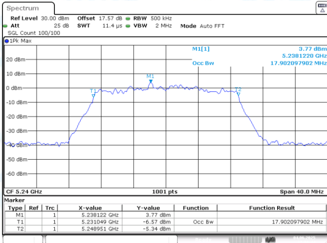
11AC20MIMO-Ant2-5240
