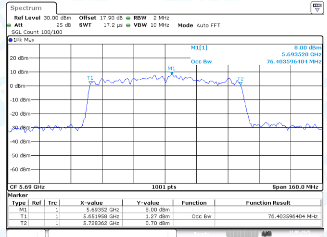
11AC80MIMO-Ant1-5690
