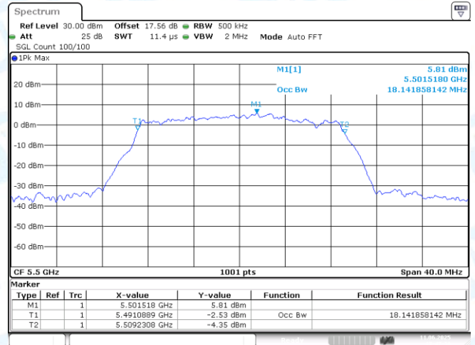
11AC20MIMO-Ant1-5500
