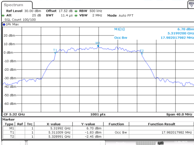
11AC20MIMO-Ant2-5320
