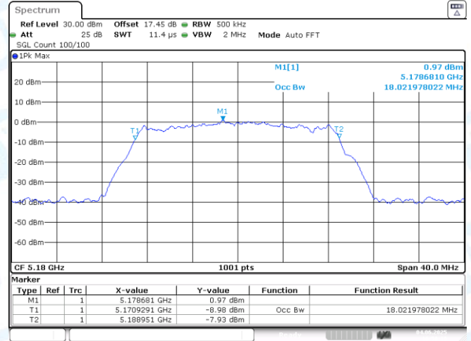
11AC20MIMO-Ant1-5180
