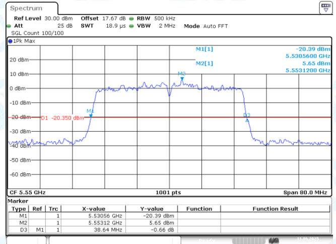
11AC40MIMO-Ant2-5550
