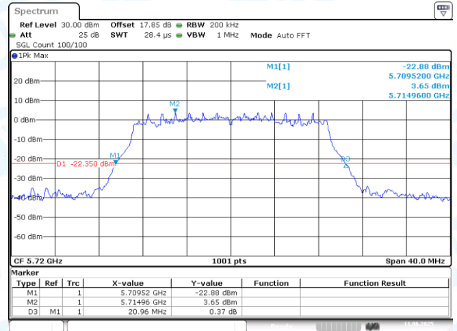
11AC20MIMO-Ant2-5720
