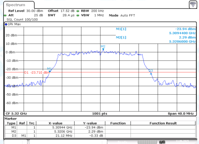
11AC20MIMO-Ant2-5320
