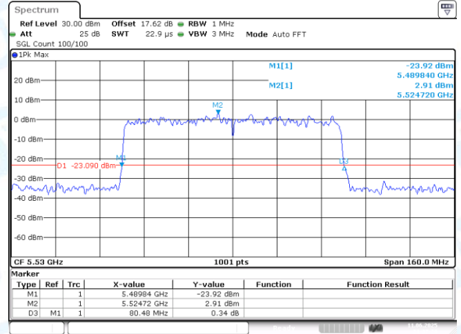
11AX80MIMO-Ant2-5530
