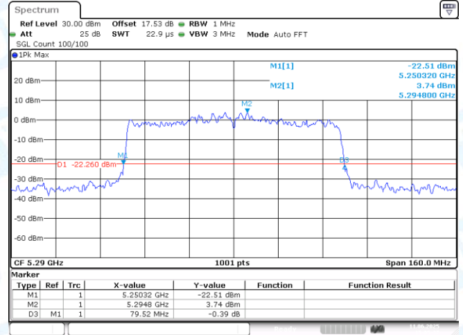
11AC80MIMO-Ant2-5290
