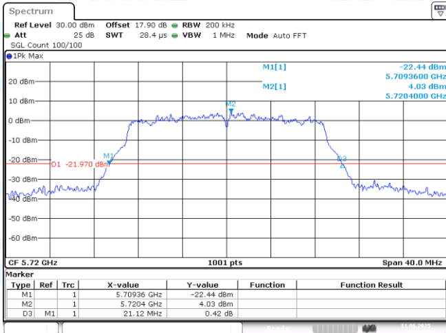
11AC20MIMO-Ant1-5720
