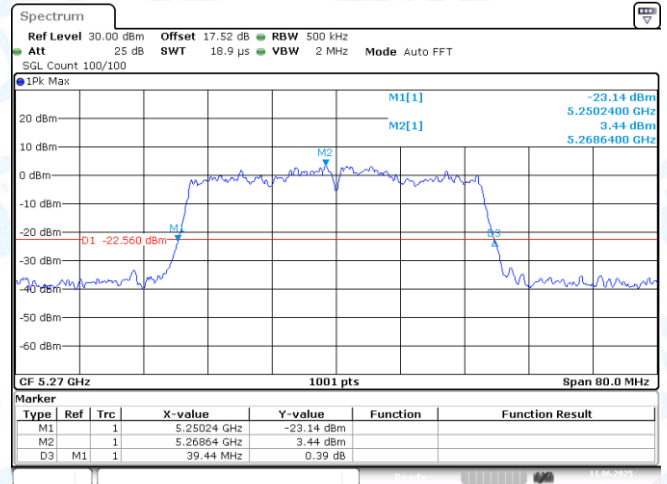
11AC40MIMO-Ant2-5270
