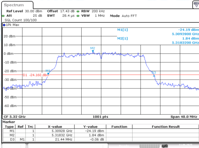
11AC20MIMO-Ant1-5320
