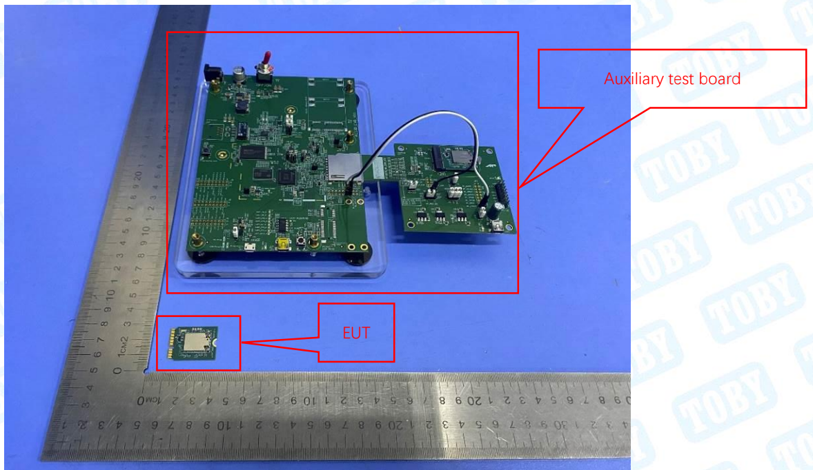
Photo 6 Appearance of EUT
