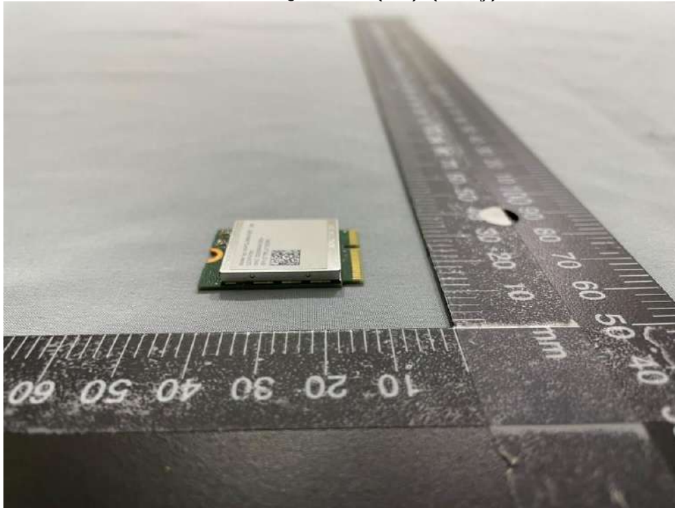
Outview: WNFQ-268AXI(BT) (E key) Pic 7
