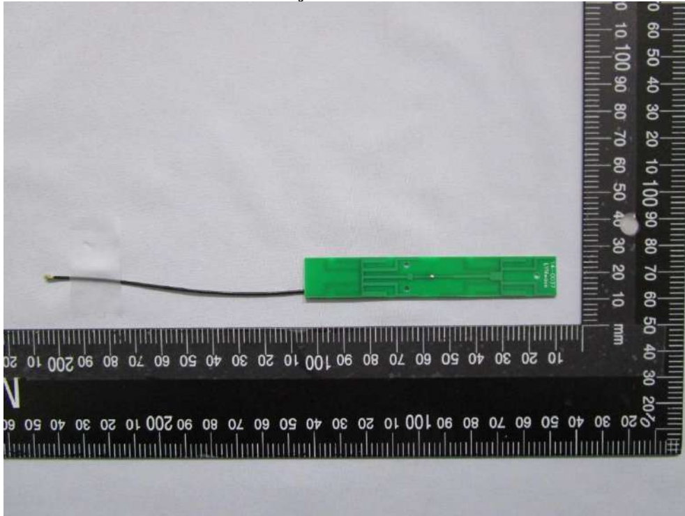
Accessory: AD-503AX Pic 1
