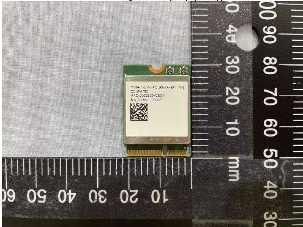
Outview: WNFQ-268AXI(BT) (E key) Pic 1
