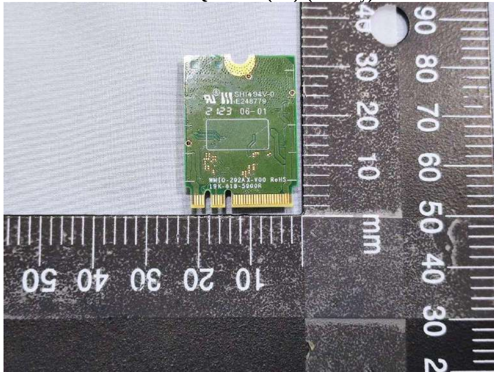
Outview: WNFQ-268AXI(BT) (A-E key) Pic 7
