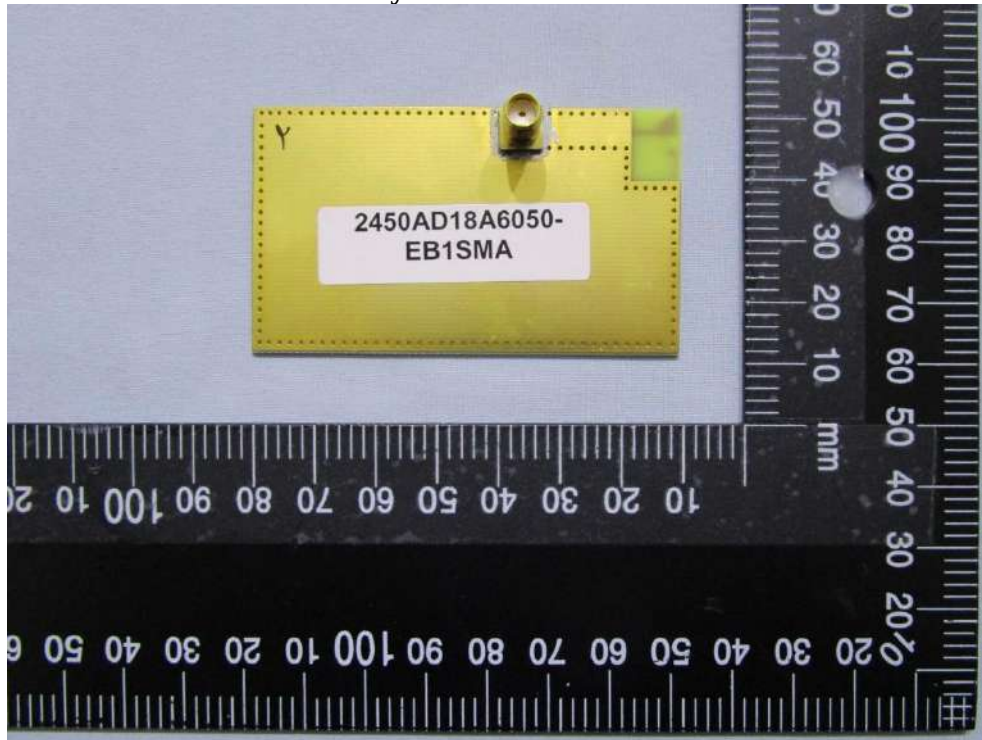
Accessory: 2450AD18A6050 Pic 3
