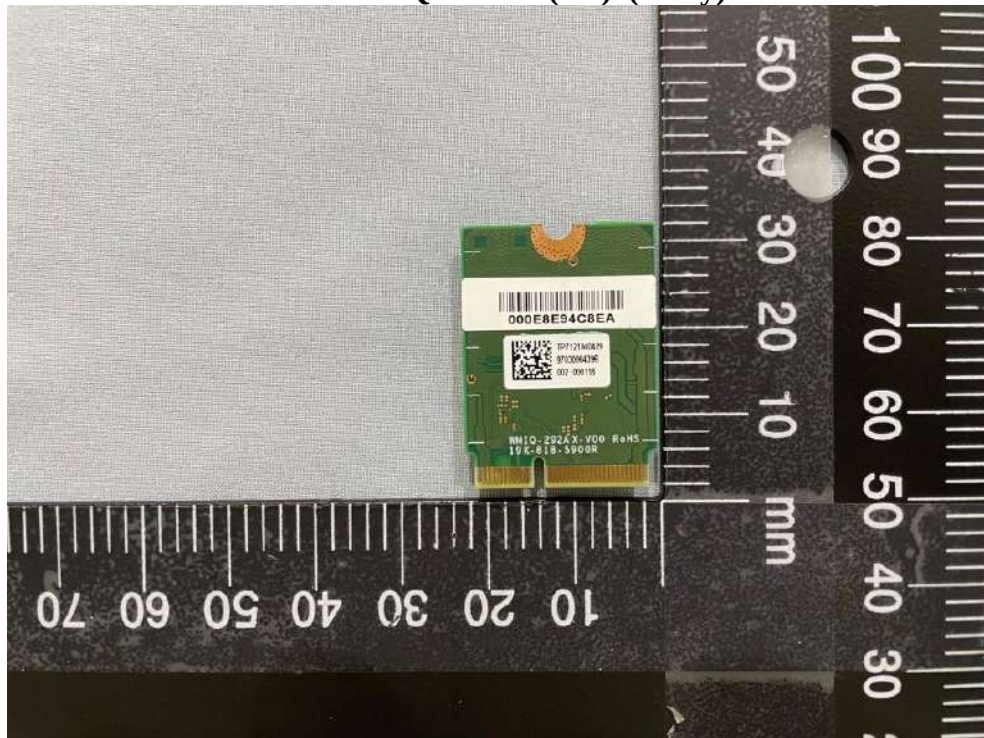
Outview: WNFQ-268AXI(BT) (E key) Pic 2
