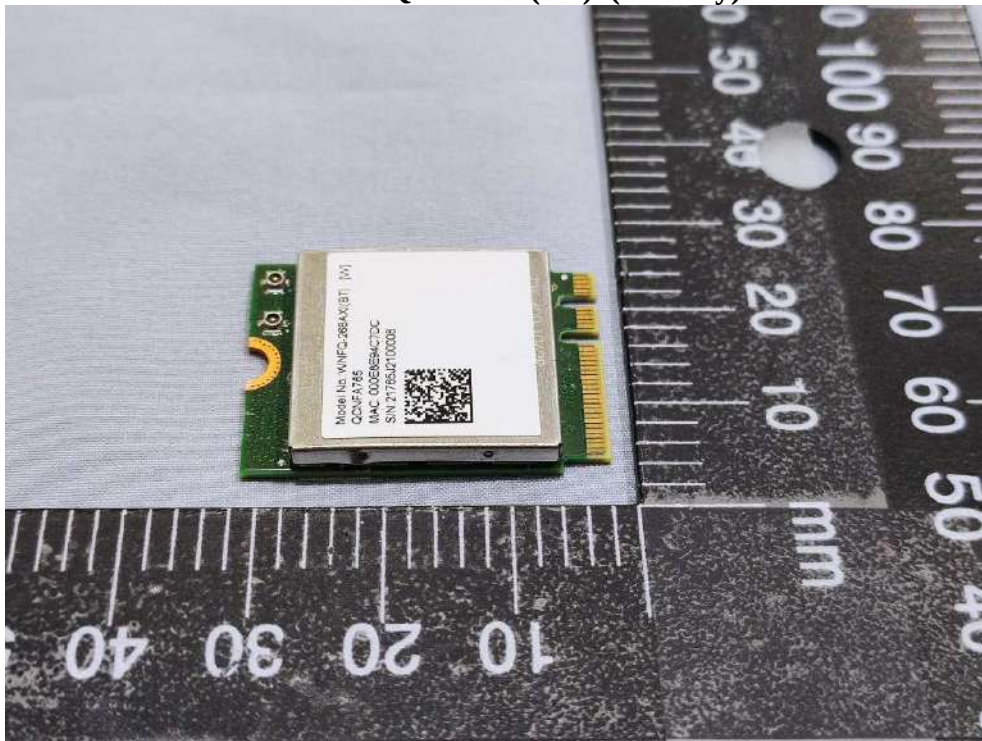
Outview: WNFQ-268AXI(BT) (A-E key) Pic 2
