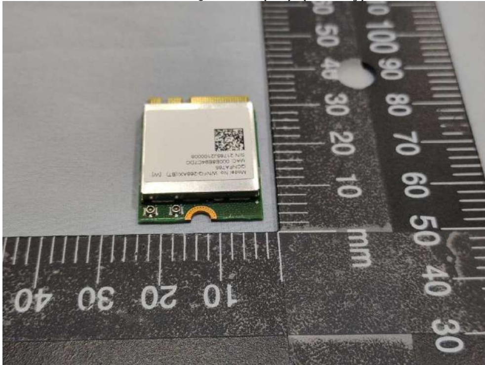
Outview: WNFQ-268AXI(BT) (A-E key) Pic 3
