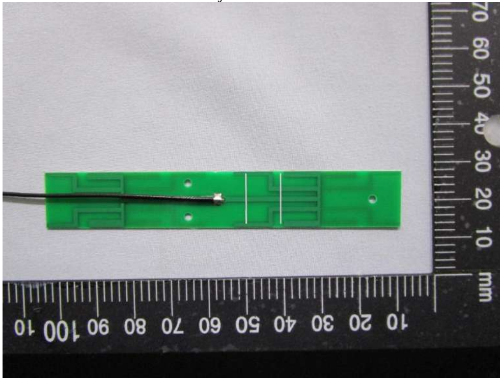
Accessory: AD-503AX Pic 3
