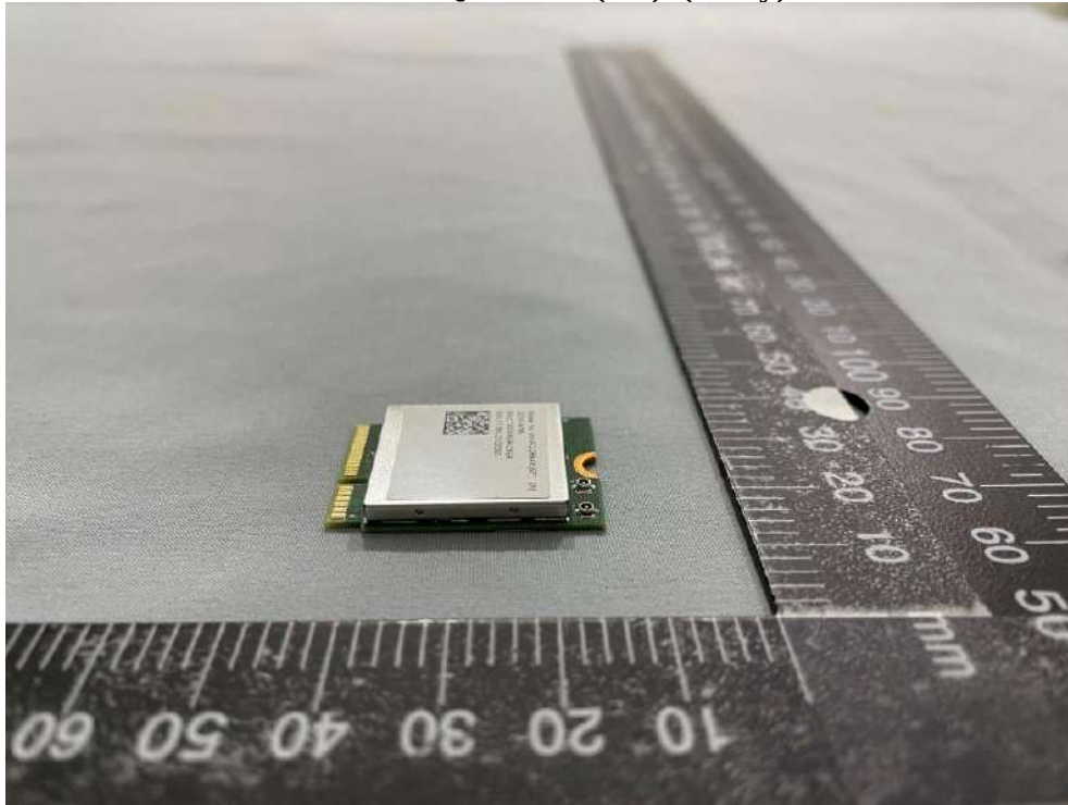
Outview: WNFQ-268AXI(BT) (E key) Pic 5
