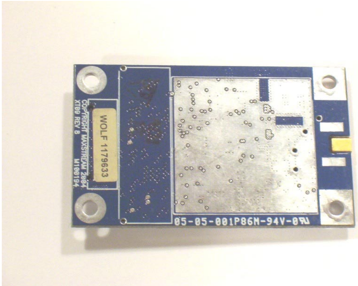
Photo 2: MaxStream RF Module – Rear View
