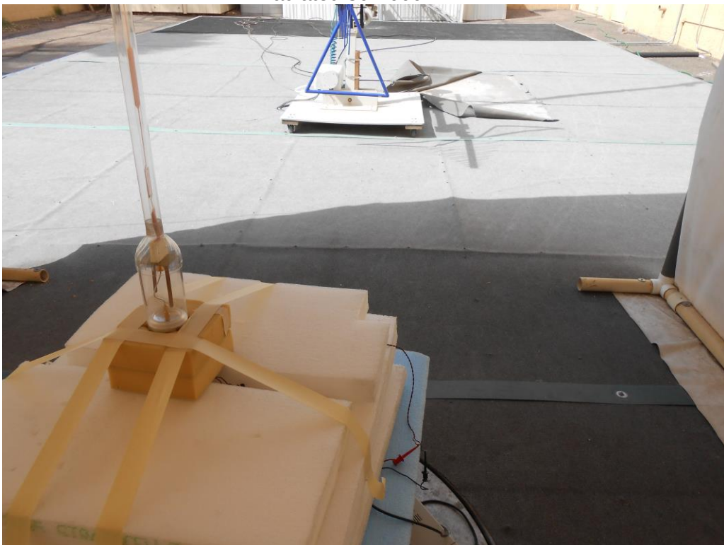
Radiated 30-1000 MHz
