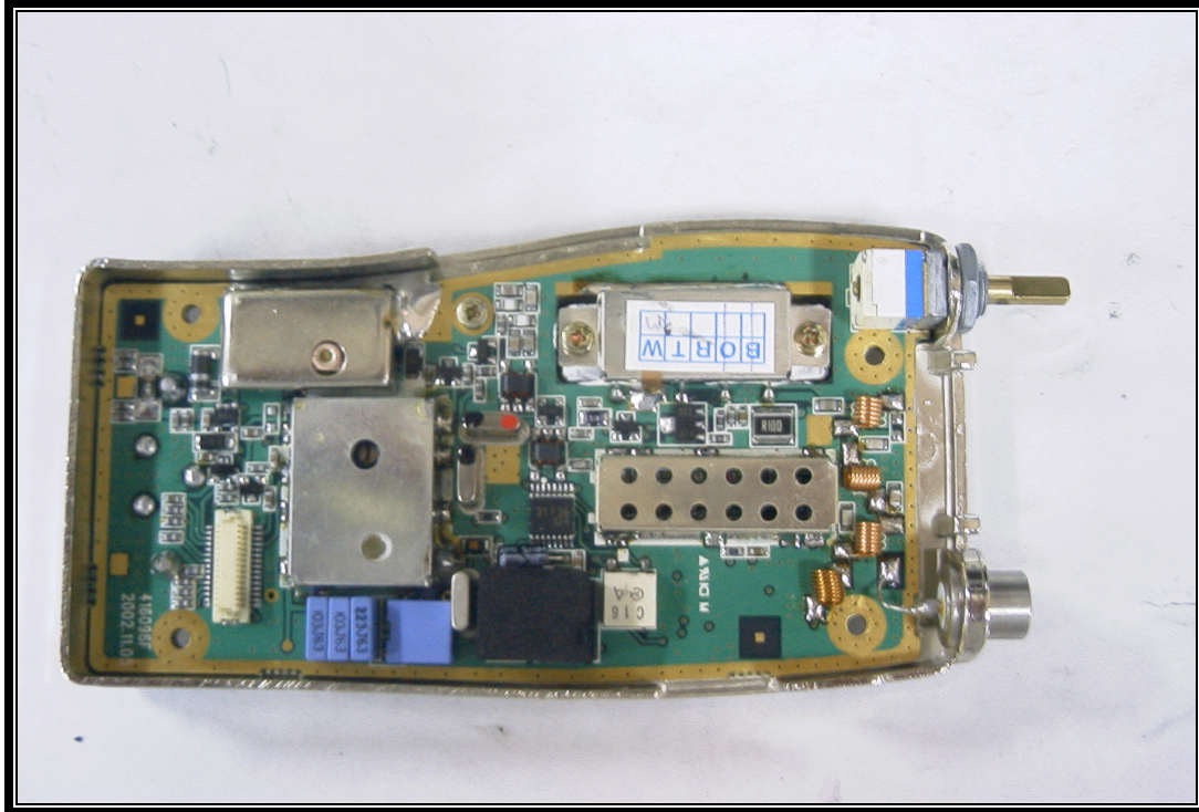
PHOTOGRAPH 13: RF PCB FRONT SIDE
