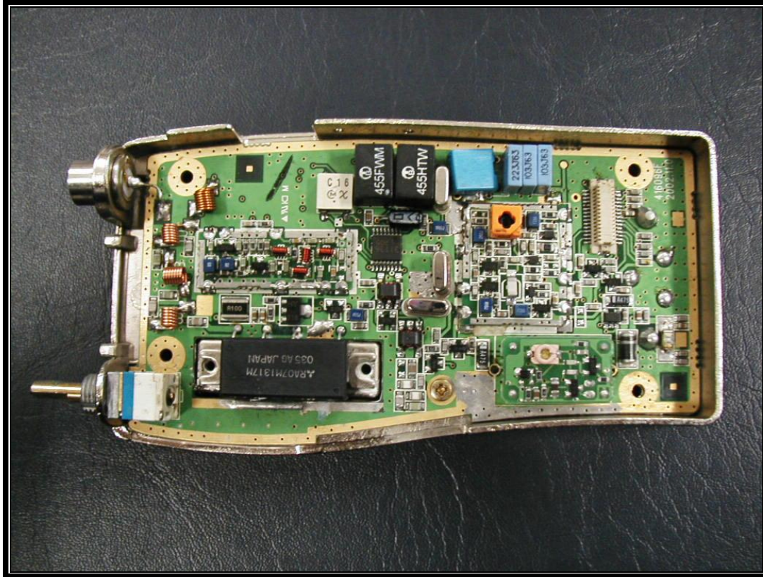
PHOTOGRAPH 14: RF PCB FRONT SIDE WITHOUT SHIELDS
