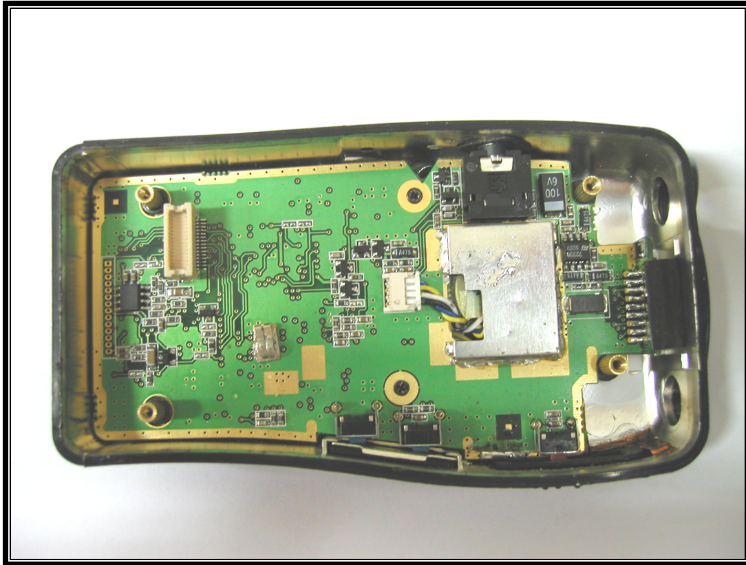
PHOTOGRAPH 10: DIGITAL PCB INSIDE FRONT CASE
