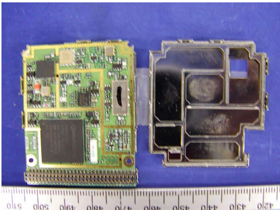
Transceiver - Shielding Off View II
