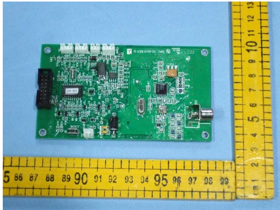
Figure 1 Receiver of the EUT-Inside View
