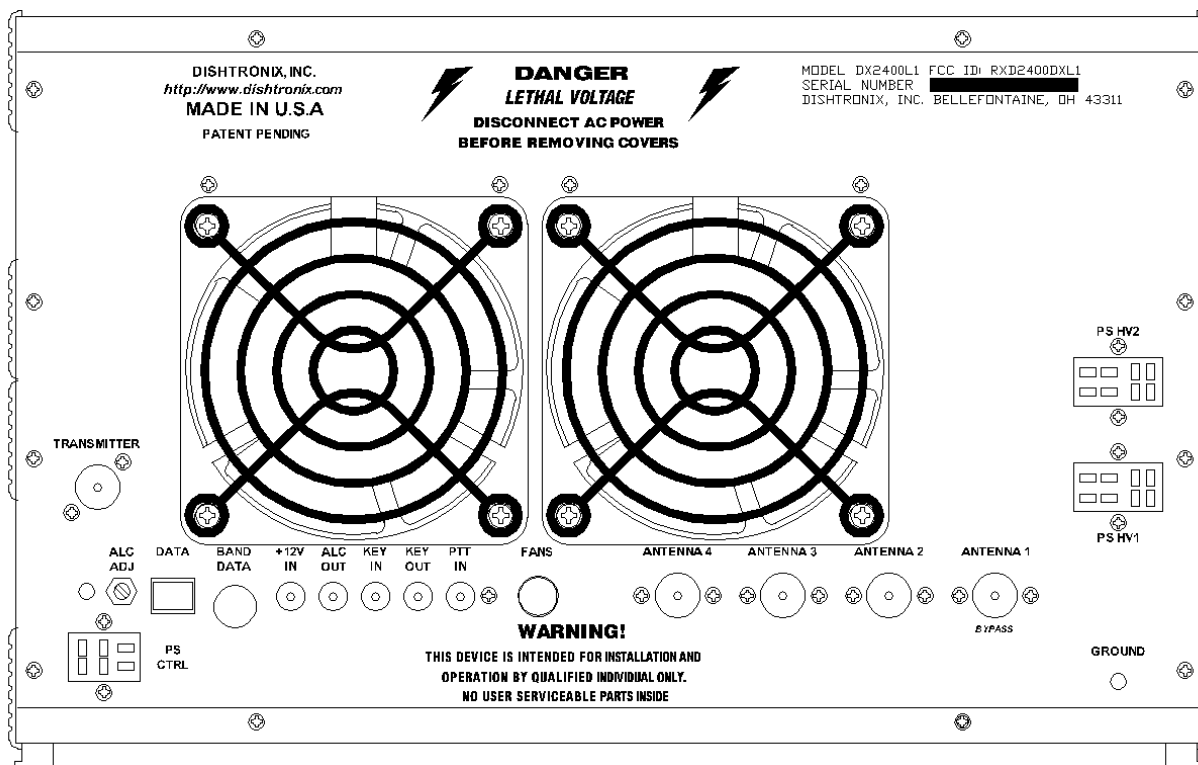
Figure 2. FCC ID Label Placement Drawing.
