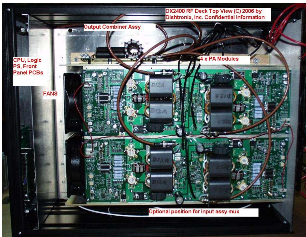
Figure 3. RF Deck Inside View (Top)
