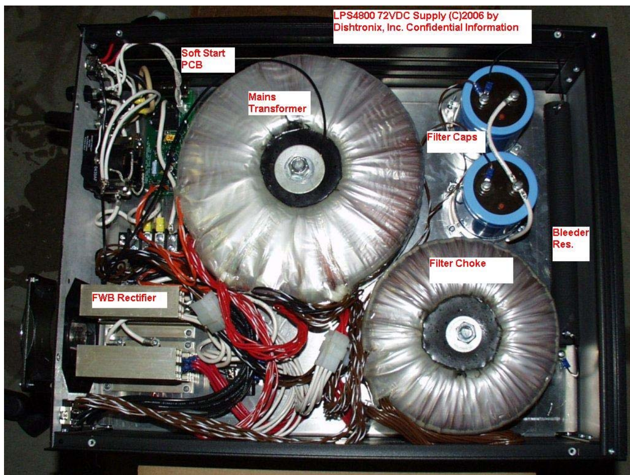
Figure 5. LPS4800 72VDC Power Supply Inside View (Top)
