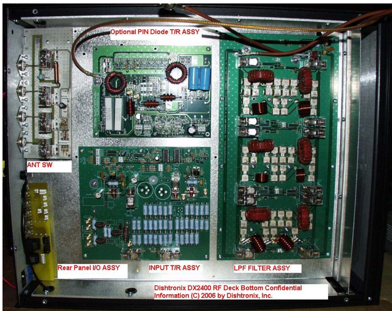
Figure 4. RF Deck Inside View (Bottom)
