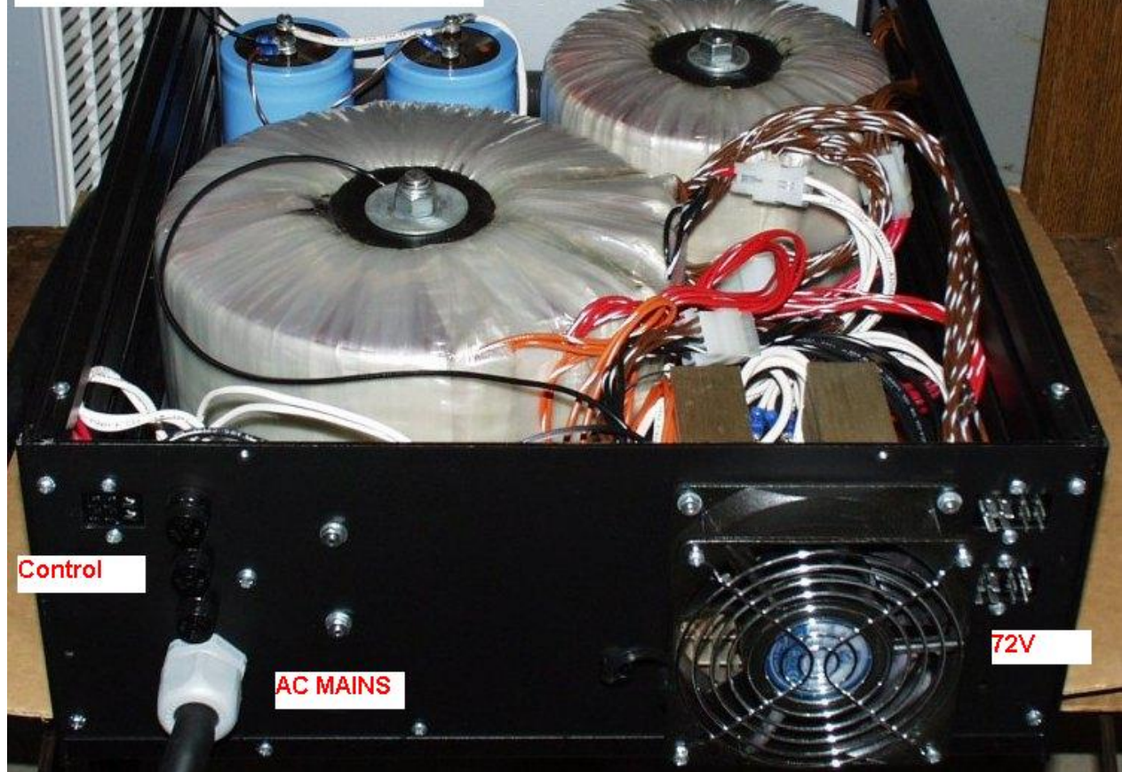
Figure 6. LPS4800 Power Supply Rear View (Top Cover Removed)
