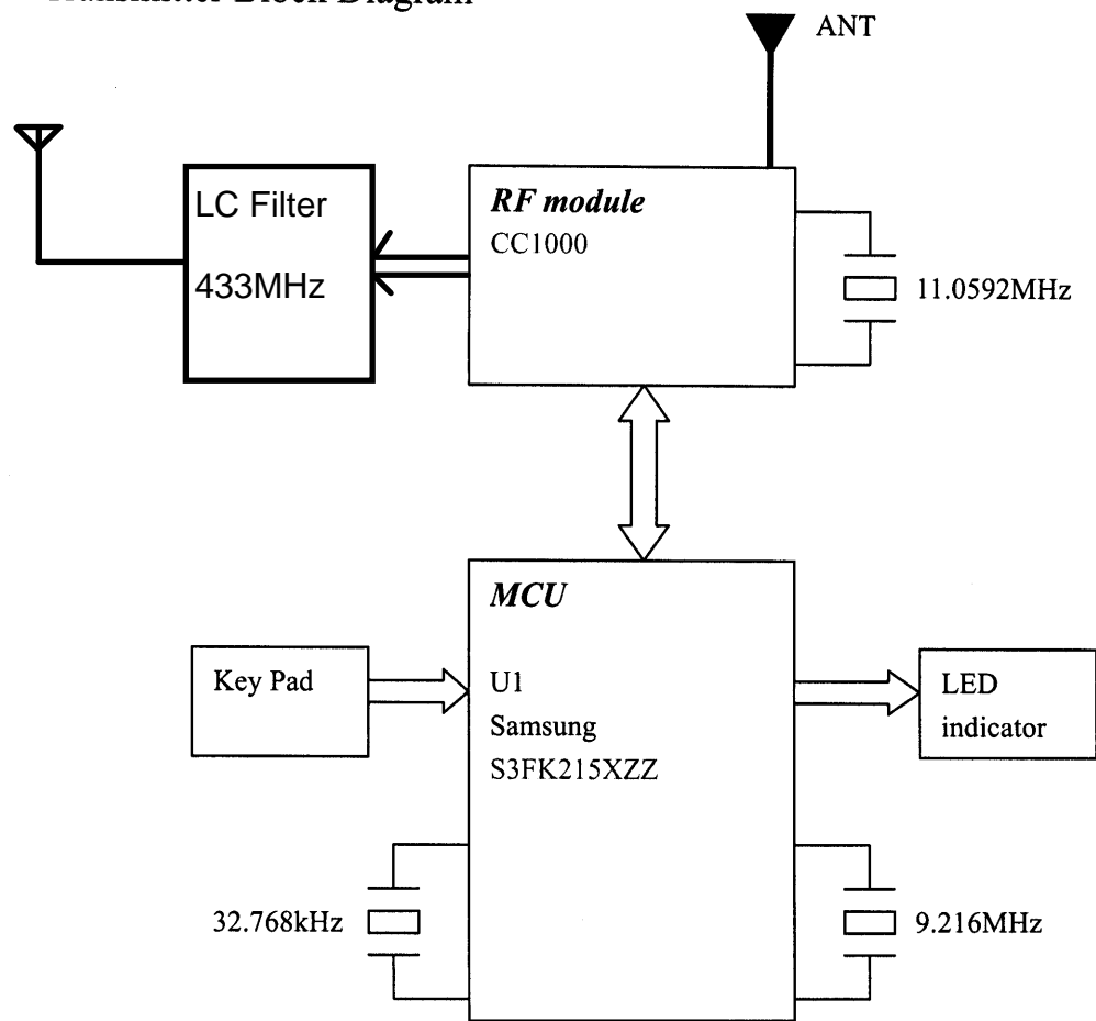
Transmitter Block Diagram
