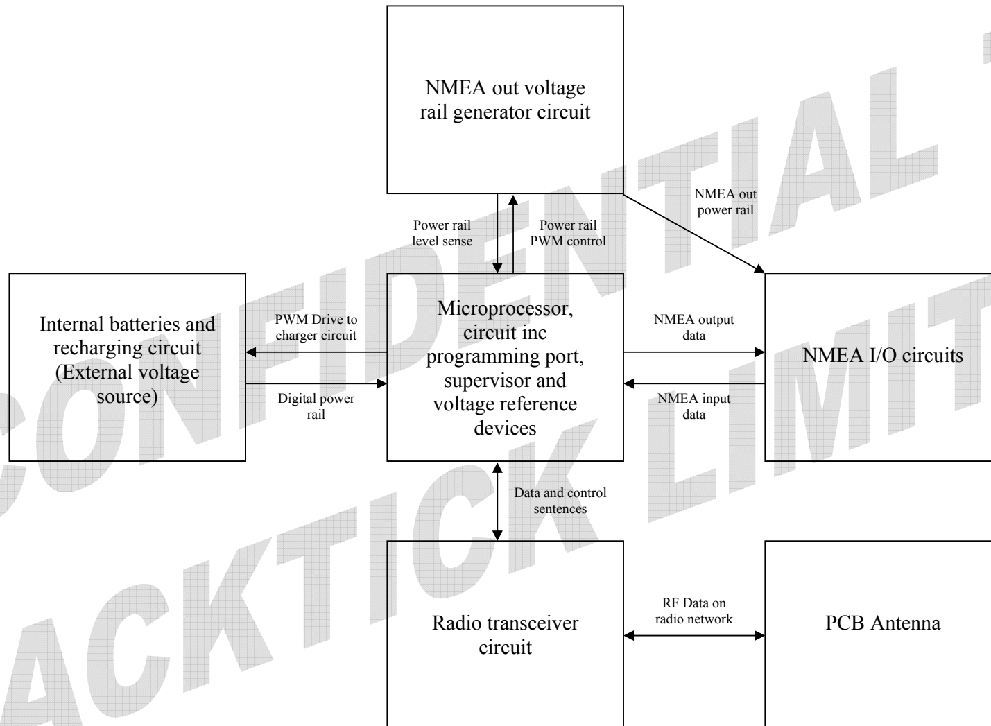
Tacktick Limited T122 NMEA Block Diagram
