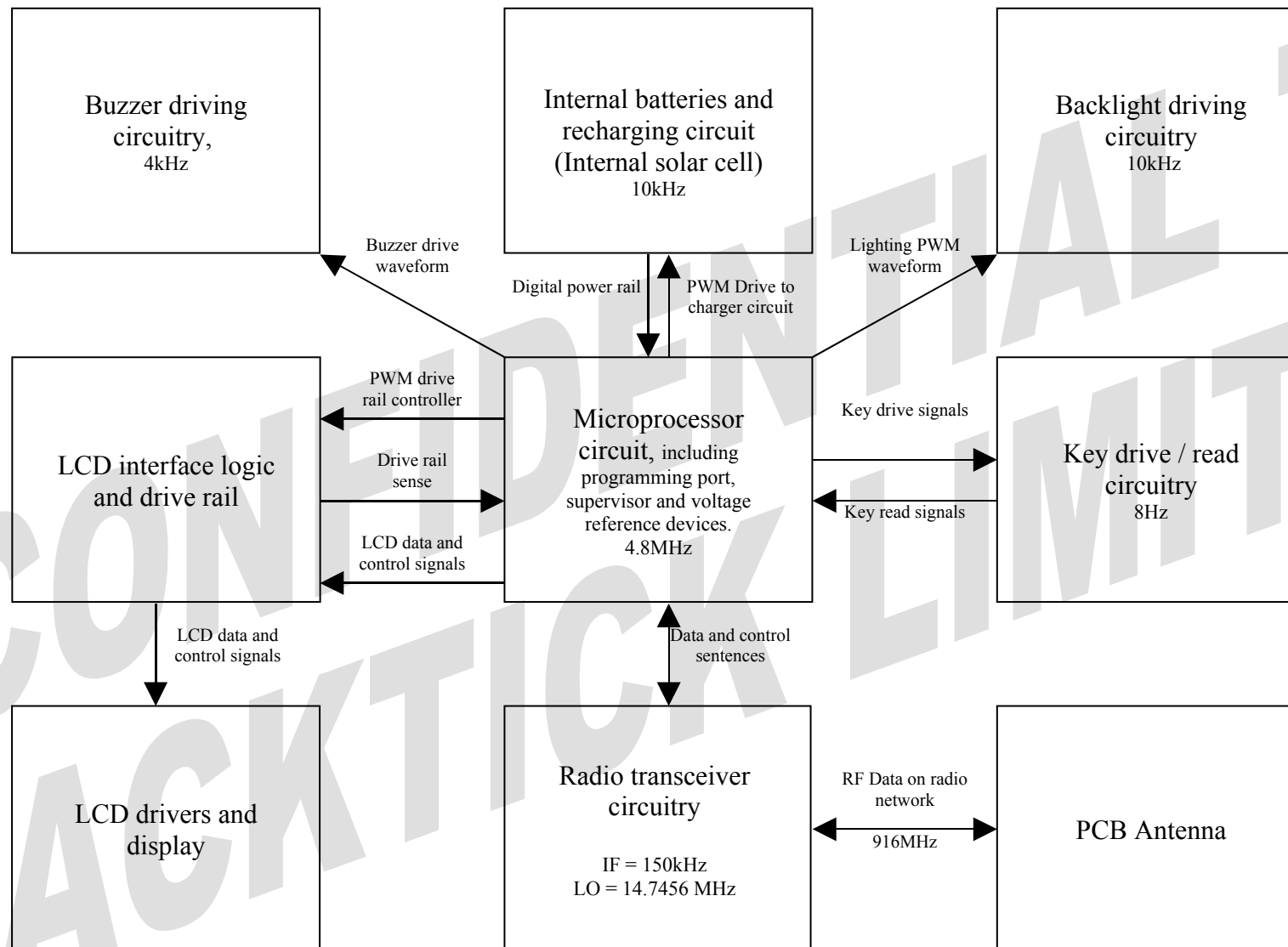
Tacktick Limited T113 Remote Display Block Diagram
