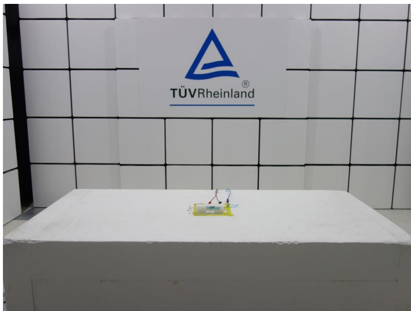
Photograph 2: Test Setup for Spurious Emissions (Front View 2)
