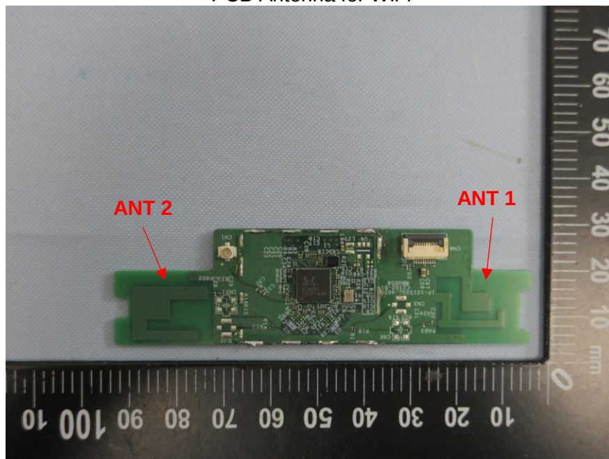
PCB Antenna for WiFi
