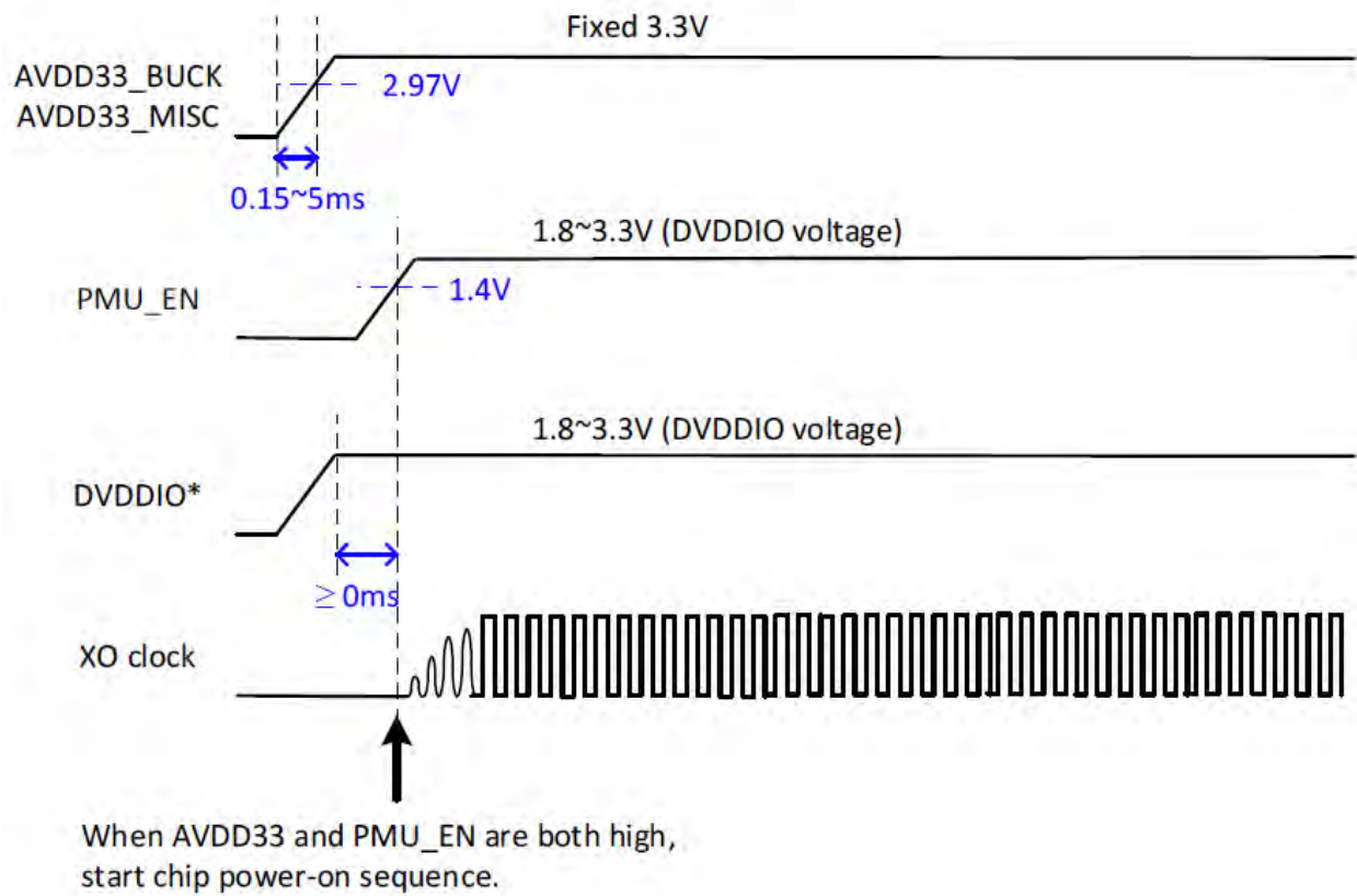
Figure 2 Power Sequence
