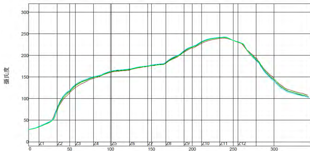
Figure 3 Soldering Specification
