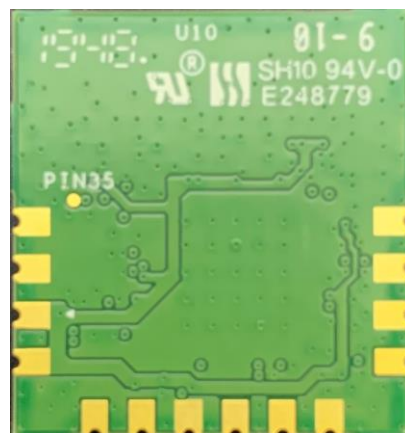
Figure 4 Bottom Side Photo
