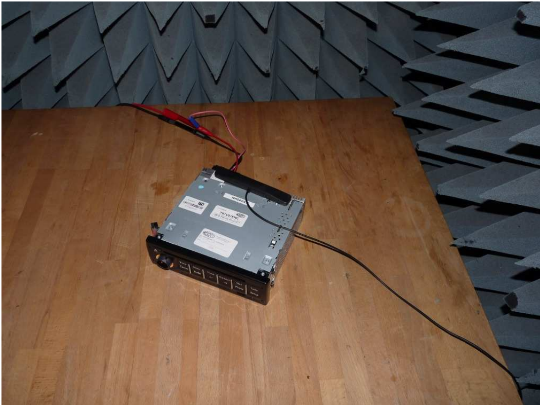
Photo 1: Setup for radiated measurements below 30 MHz
