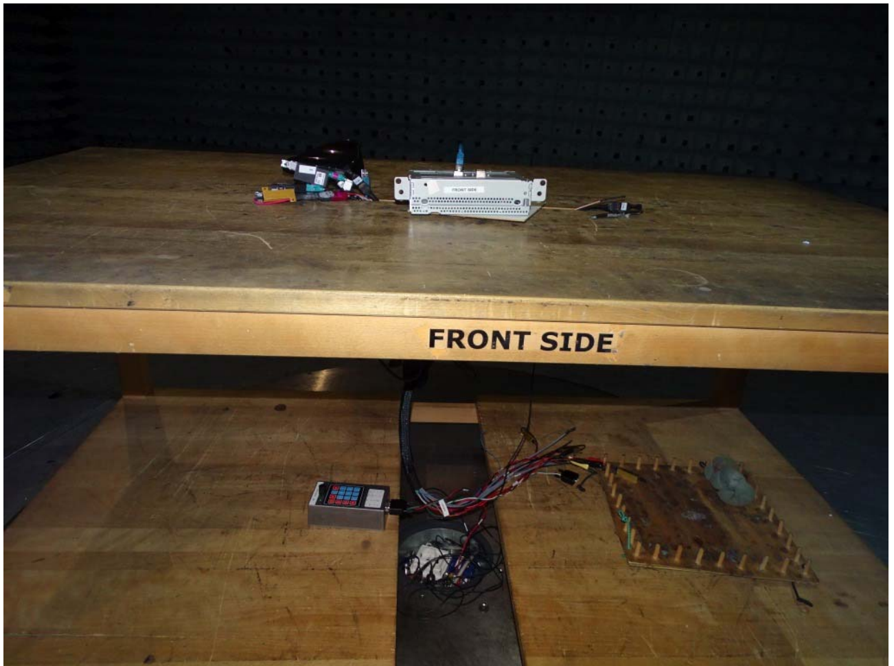
Photo 1: Test setup for radiated measurements below 30 MHz, detailed view
