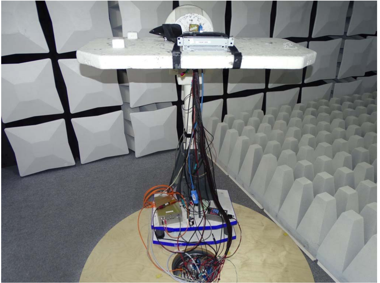
Photo 6: Test setup for radiated measurements in fully-anechoic chamber, detailed view
