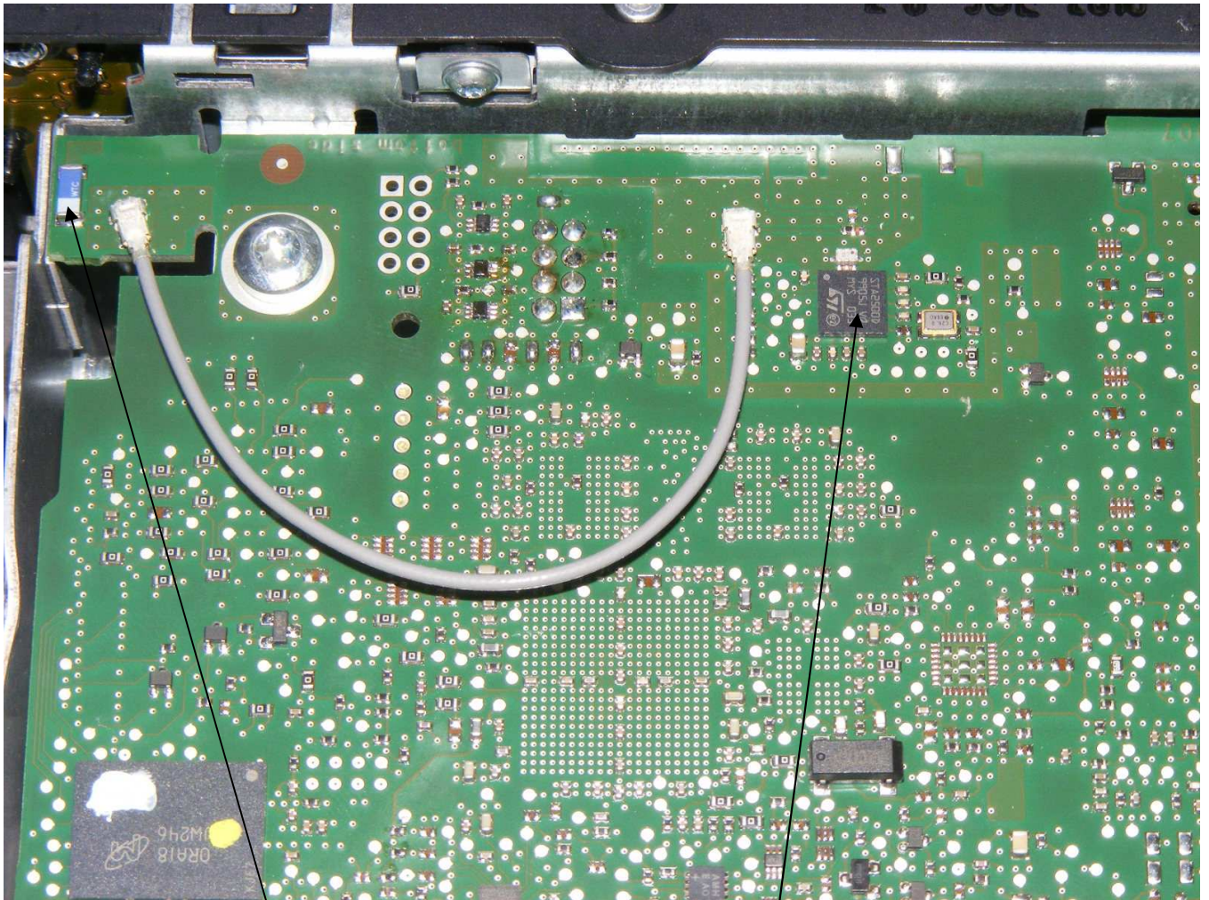
Bluetooth Antenna
