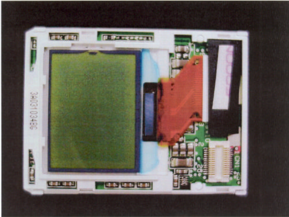
Photo 11. Display – Back
