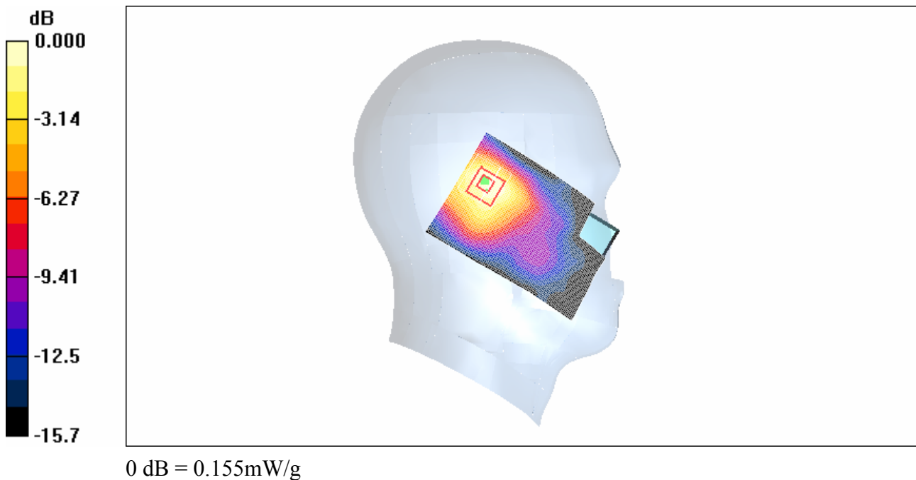
Fig.7 1900 MHz CH810
