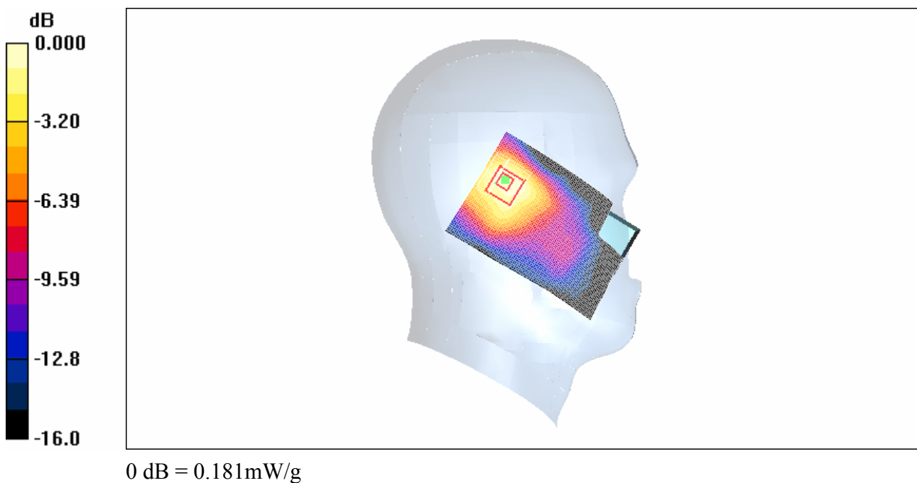
Fig.9 1900 MHz CH661
