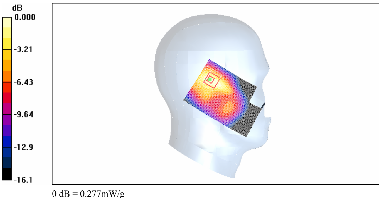
Fig. 5 1900 MHz CH512
