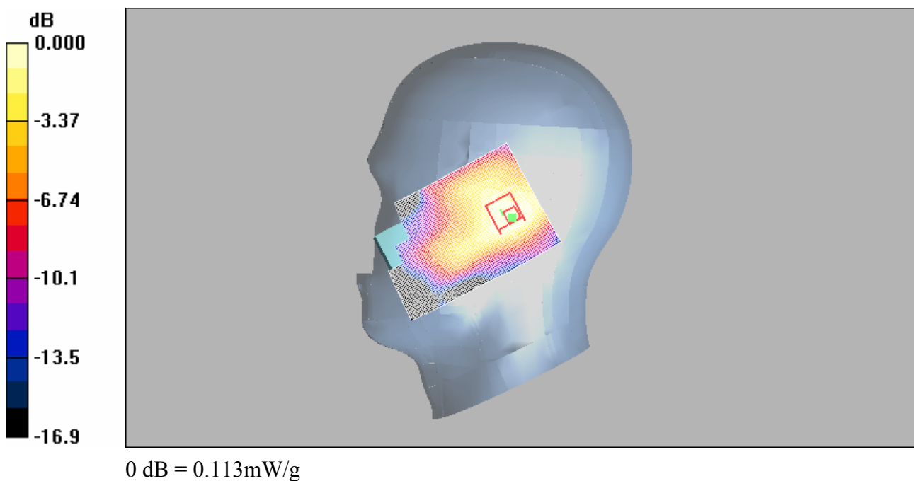
Fig. 13 1900 MHz CH810
