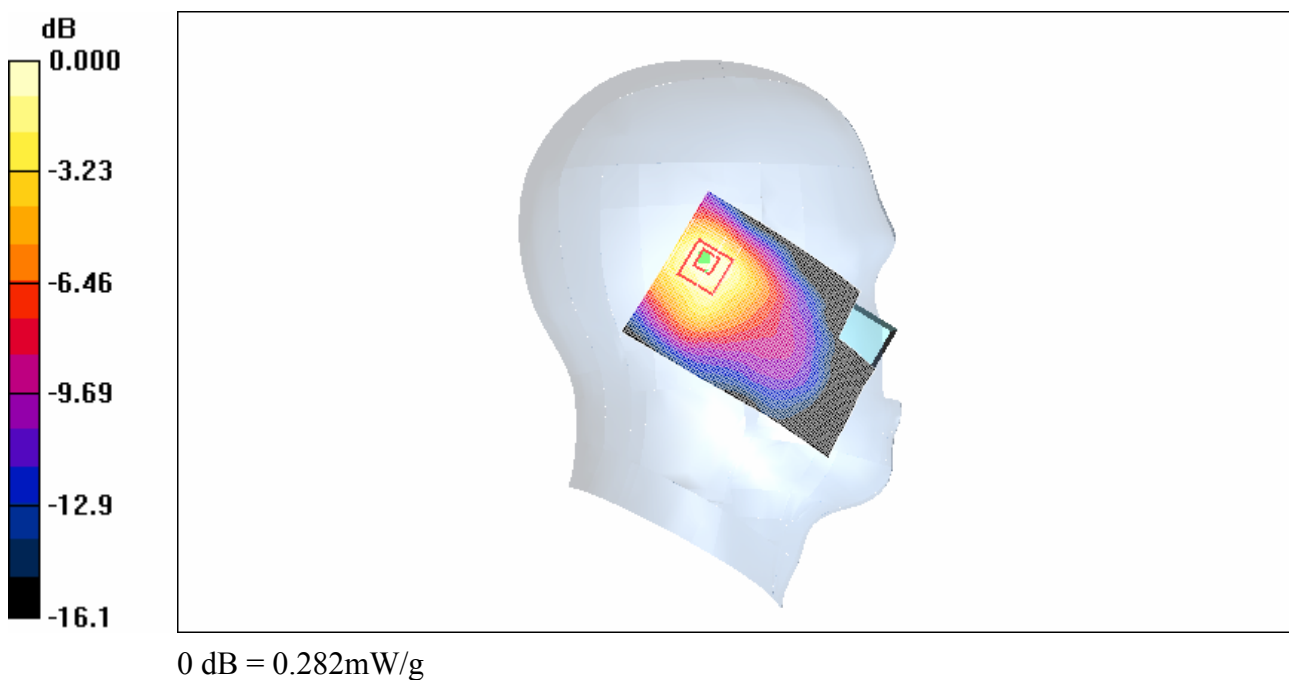
Fig. 11 1900 MHz CH512
