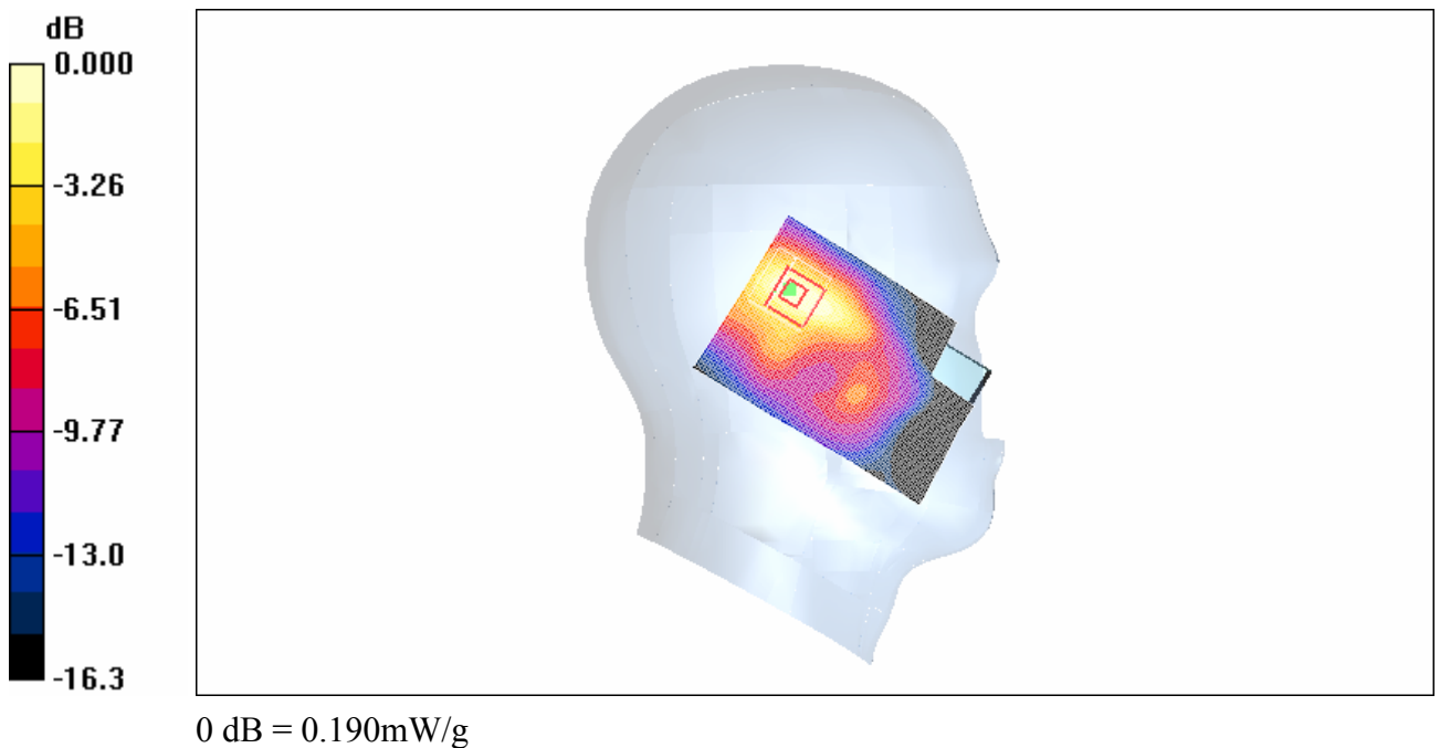
Fig. 3 1900 MHz CH661
