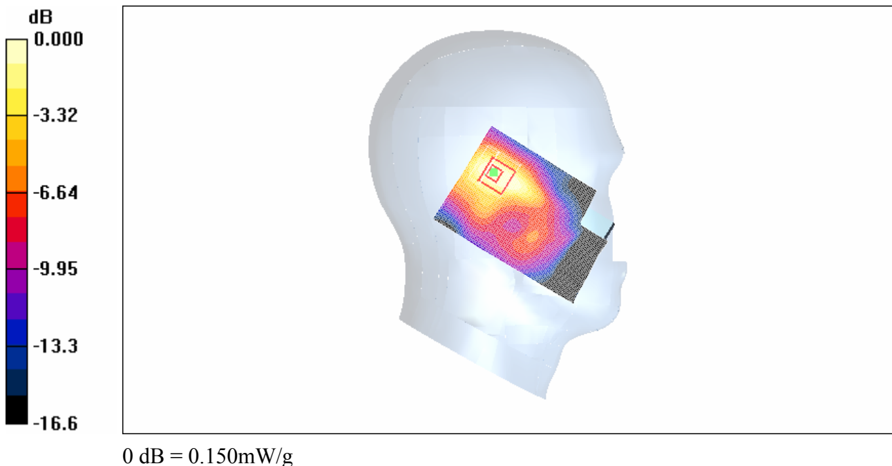
Fig. 1 1900 MHz CH810
