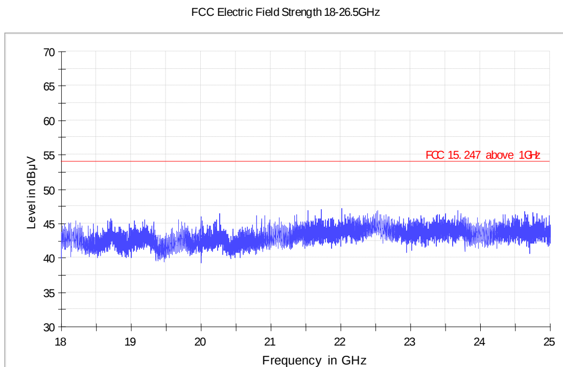
Figure 7: Test figure of spurious emissions, mode A.1, Vertical polarity (18GHz – 25GHz)
