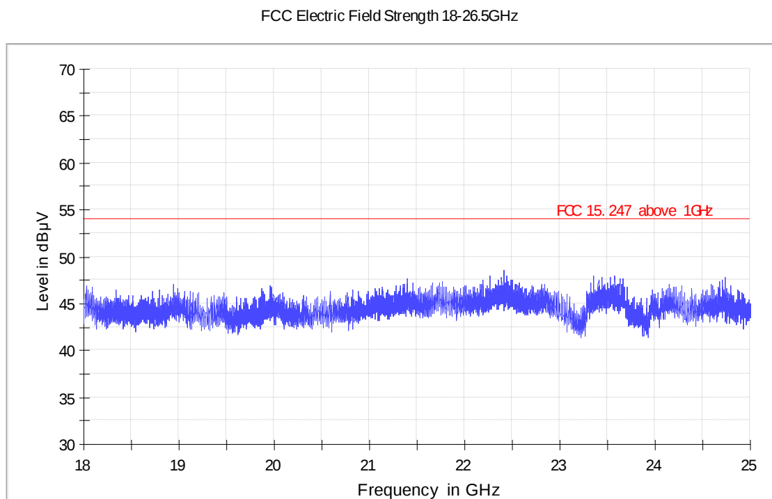
Figure 21: Test figure of spurious emissions, mode A.3, Vertical polarity (18GHz – 25GHz)
