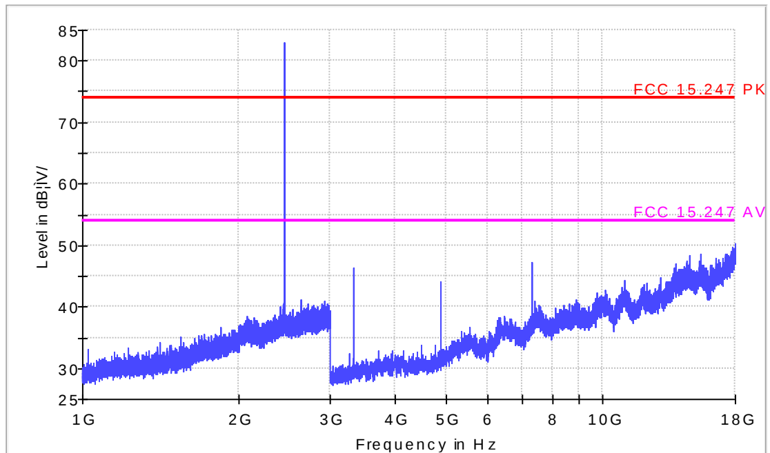
Figure 12: Test figure of spurious emissions, mode A.2, Vertical polarity (1GHz – 18GHz)
