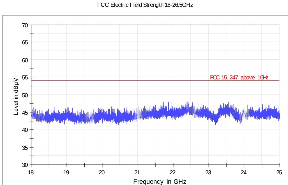
Figure 20: Test figure of spurious emissions, mode A.3, Horizontal polarity (18GHz –25GHz)
