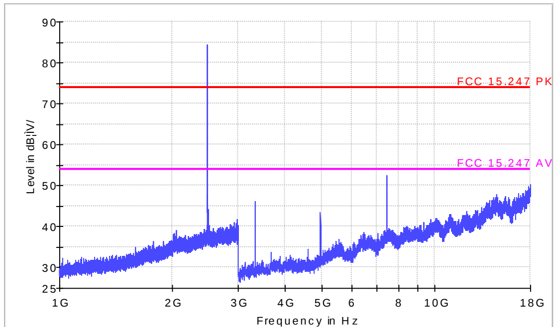
Figure 19: Test figure of spurious emissions, mode A.3, Vertical polarity (1GHz – 18GHz)
