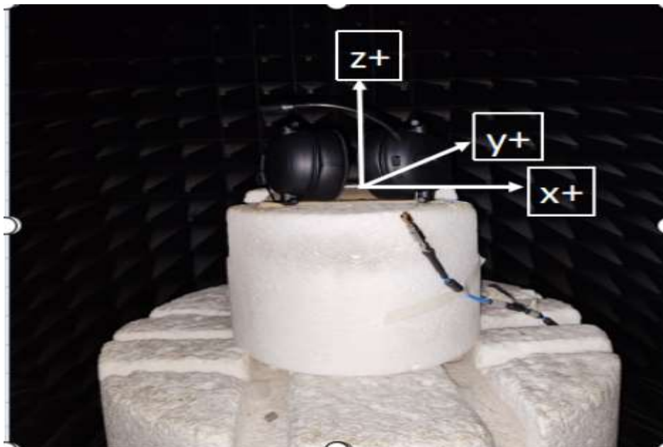
EUT SET PHOTO
