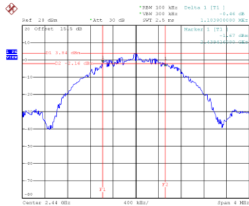
CH38 6 dB Bandwidth
