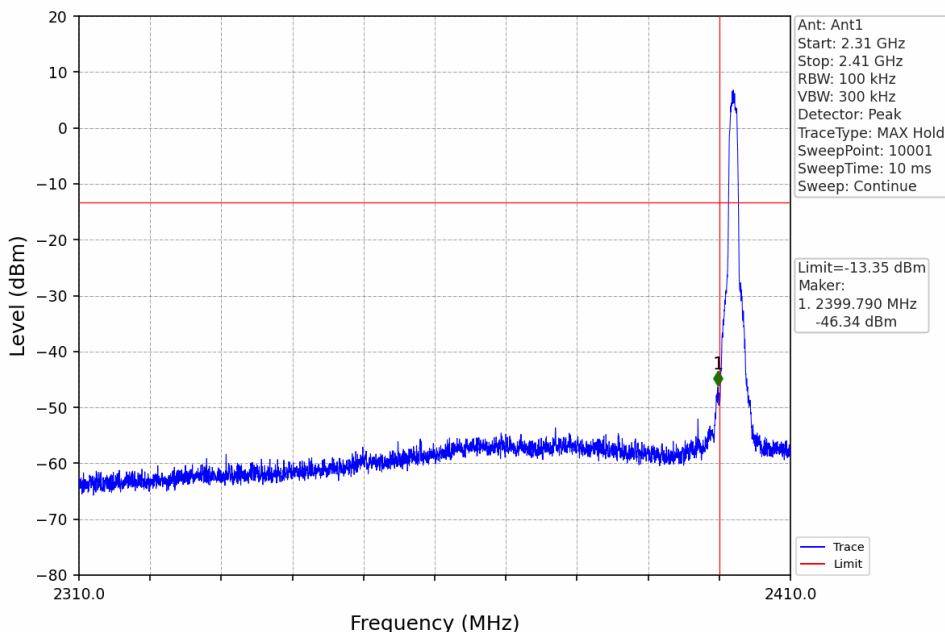
8DPSK_3DH5_LCH_2402MHz_Ant1_NTNV
