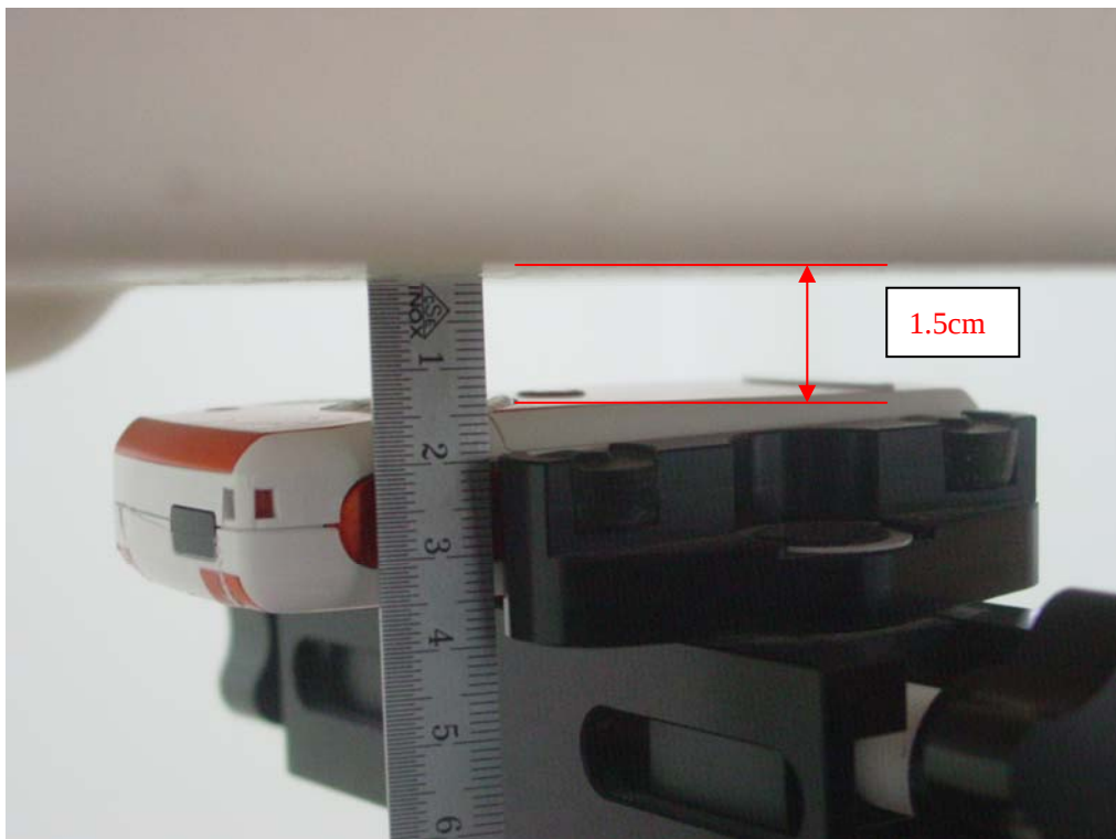
Picture B4: Body-worn Position with GPRS and Bluetooth (toward ground, the distance from handset to the bottom of the Phantom is 1.5cm)
