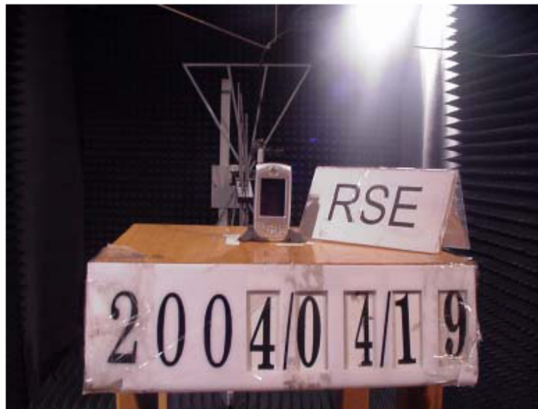
Pic2 Radiated Spurious Emission
