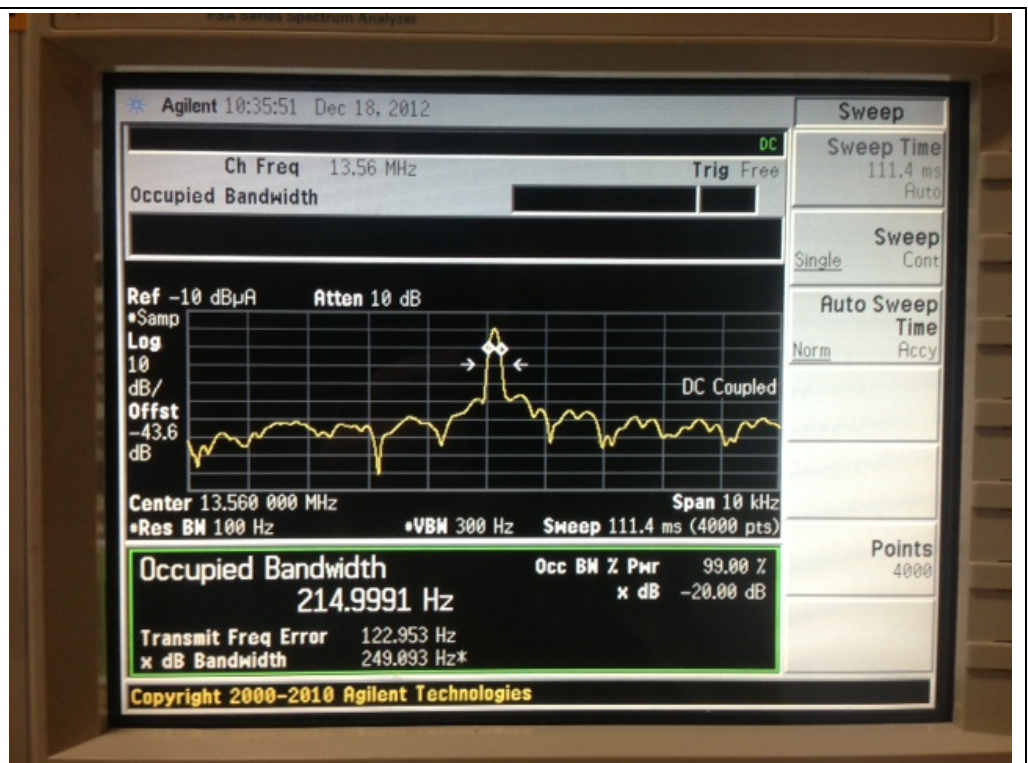
Occupied bandwidth
