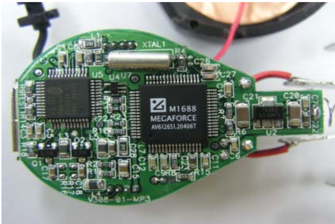
Internal of EUT – Open
