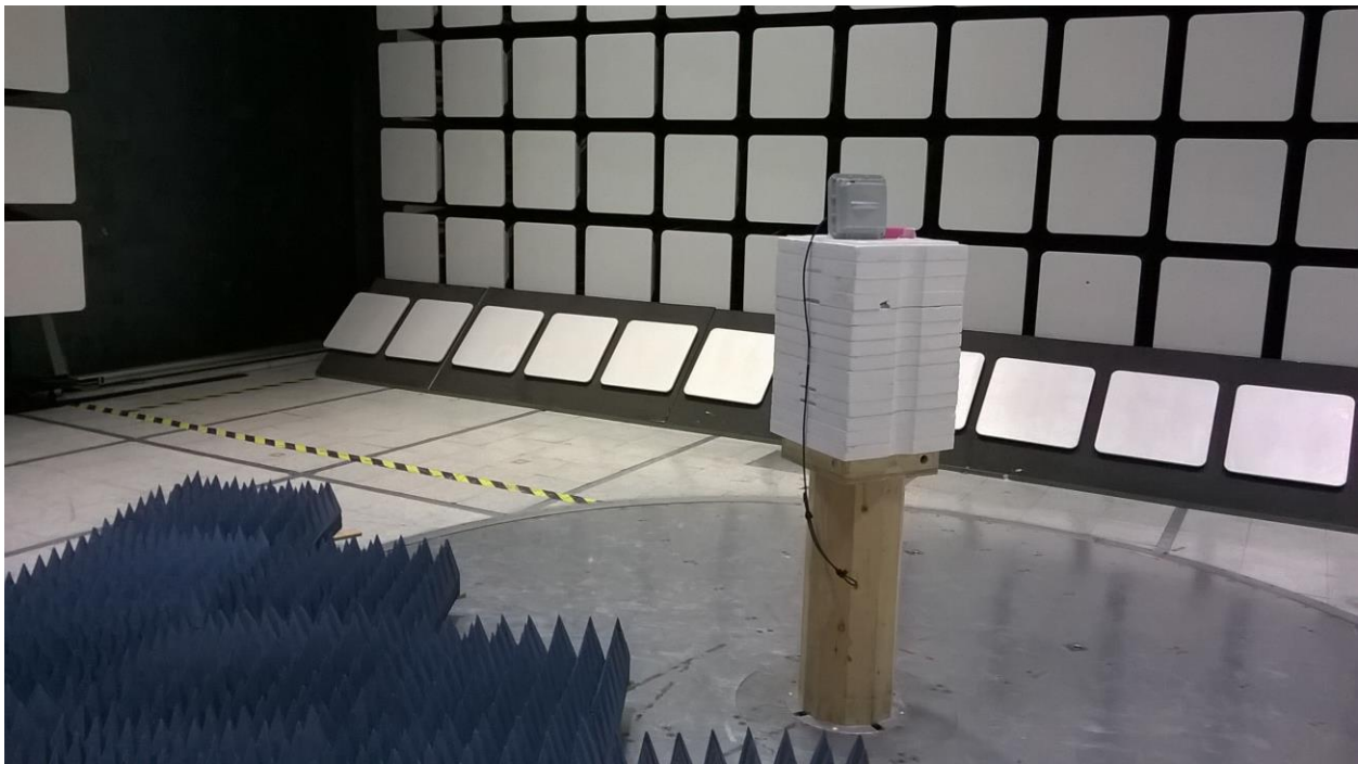
Figure 4 - 1 - 10GHz, Z-axis
