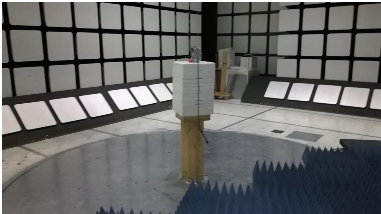
Figure 6 - 1 - 10GHz, Z-axis
