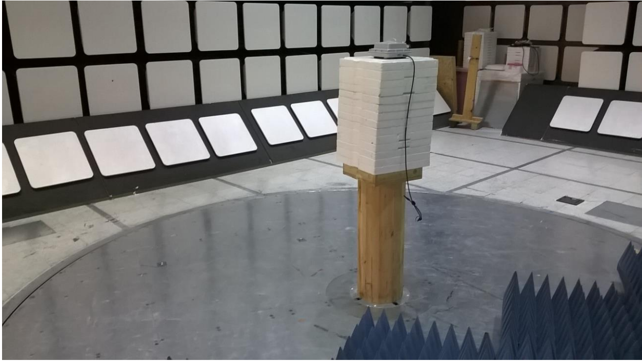
Figure 1 - 1 - 10GHz, X-axis
