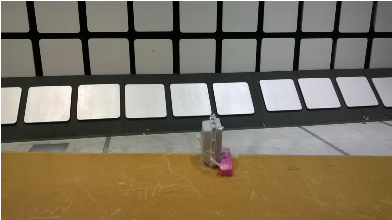
Figure 11 - 30MHz - 1GHz, Z-axis
