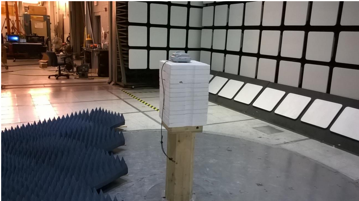
Figure 3 - 1 - 10GHz, Z-axis
