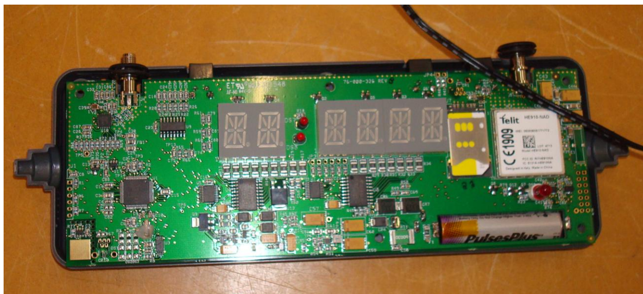
Figure 1 - Front Side
