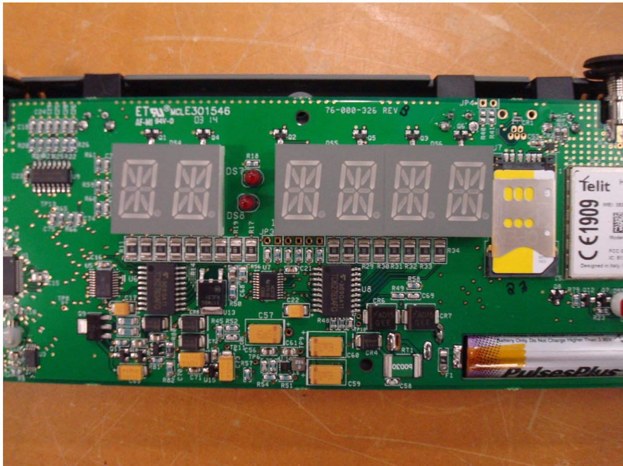
Figure 5 - Front Sid Center Detail
