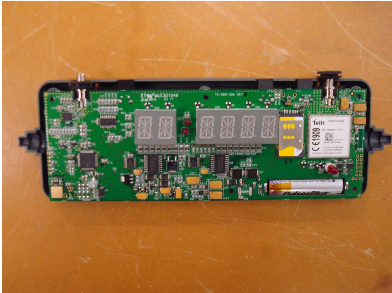
Figure 3 - Front Side
